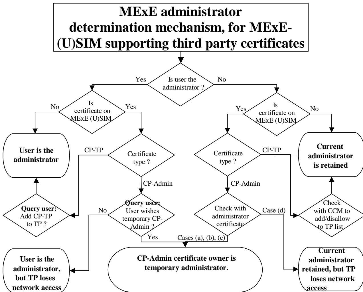
Figure 14: MExE administrator determination mechanism, for MExE-(U)SIM supporting third party certificates
