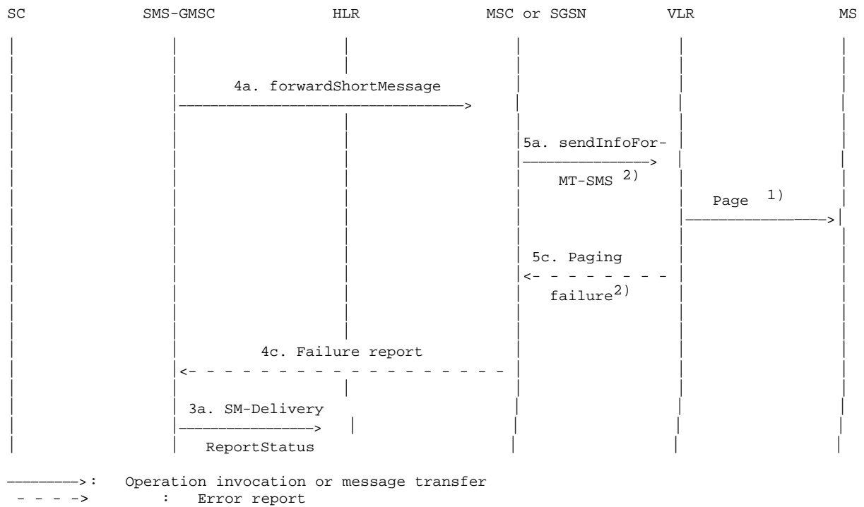
Figure 03.40/16b): "Send information for MT SMS" procedure; erroneous case: absent subscriber (e.g. IMSI DETACH or GPRS DETACH)
