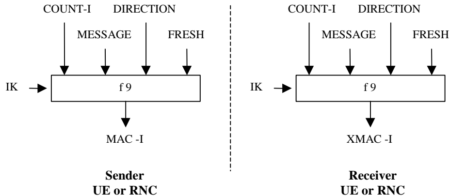
Figure 2: Derivation of MAC-I (or XMAC-I) on a signalling message
