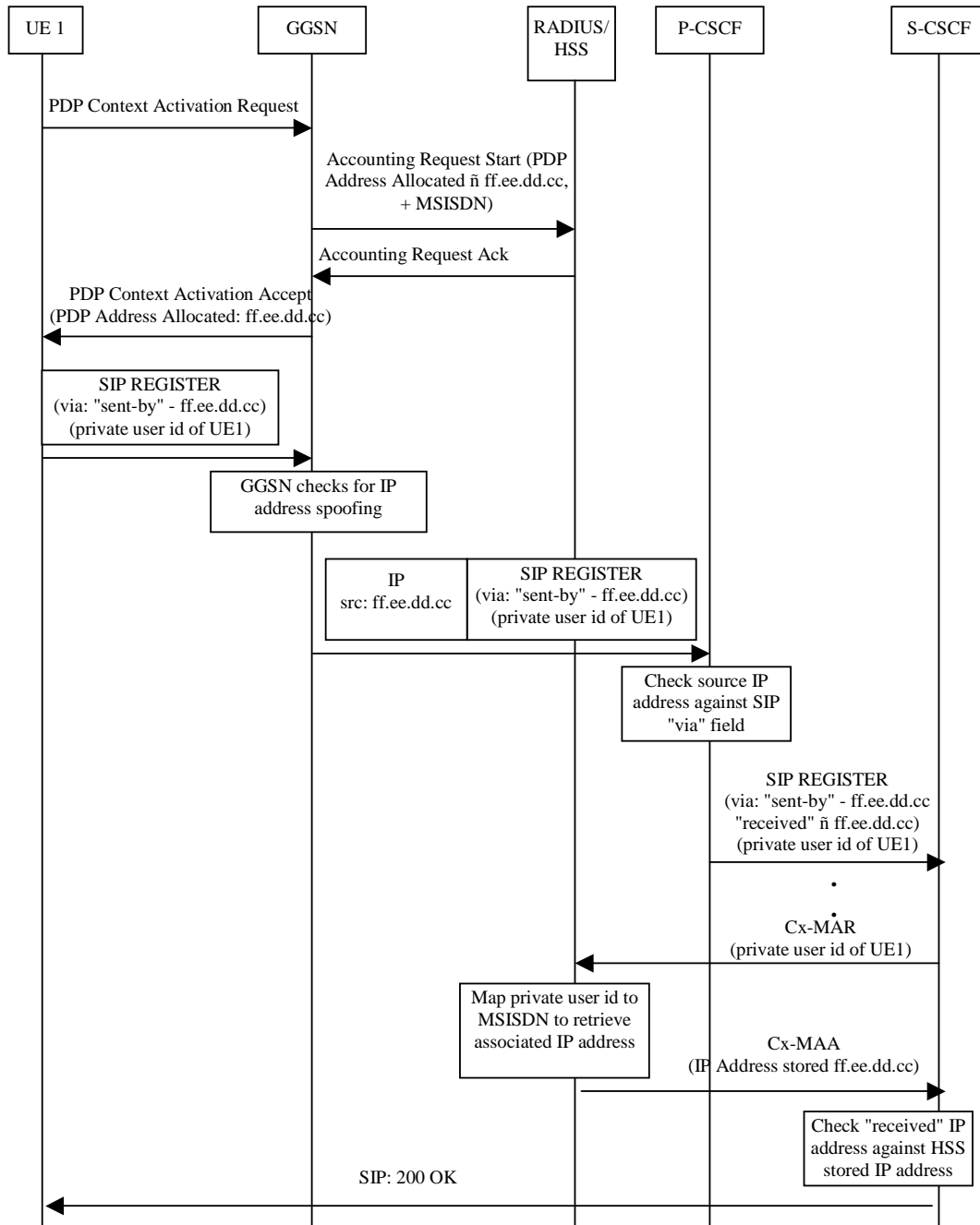
Figure 1: Message Sequence for Interim early IMS Security Solution (showing a successful registration)
