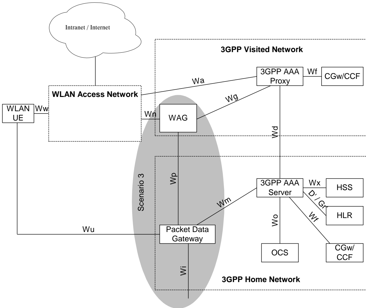
Figure 2: Roaming reference model - 3GPP PS based services provided via the 3GPP Home Network (the shaded area refers to scenario 3 functionality)
