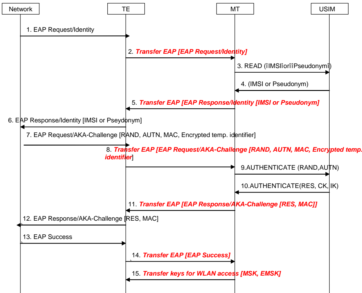
Figure 11: Full authentication with EAP AKA
