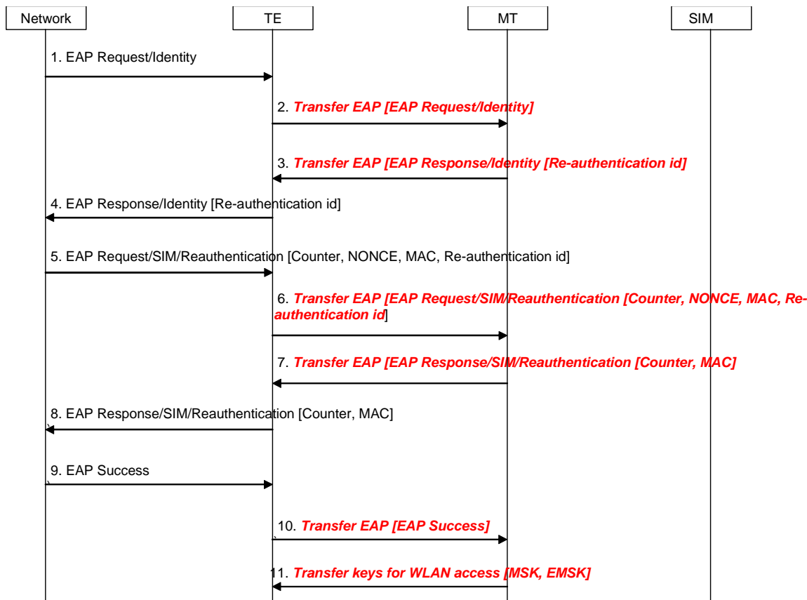
Figure 14: Fast re-authentication with EAP SIM
