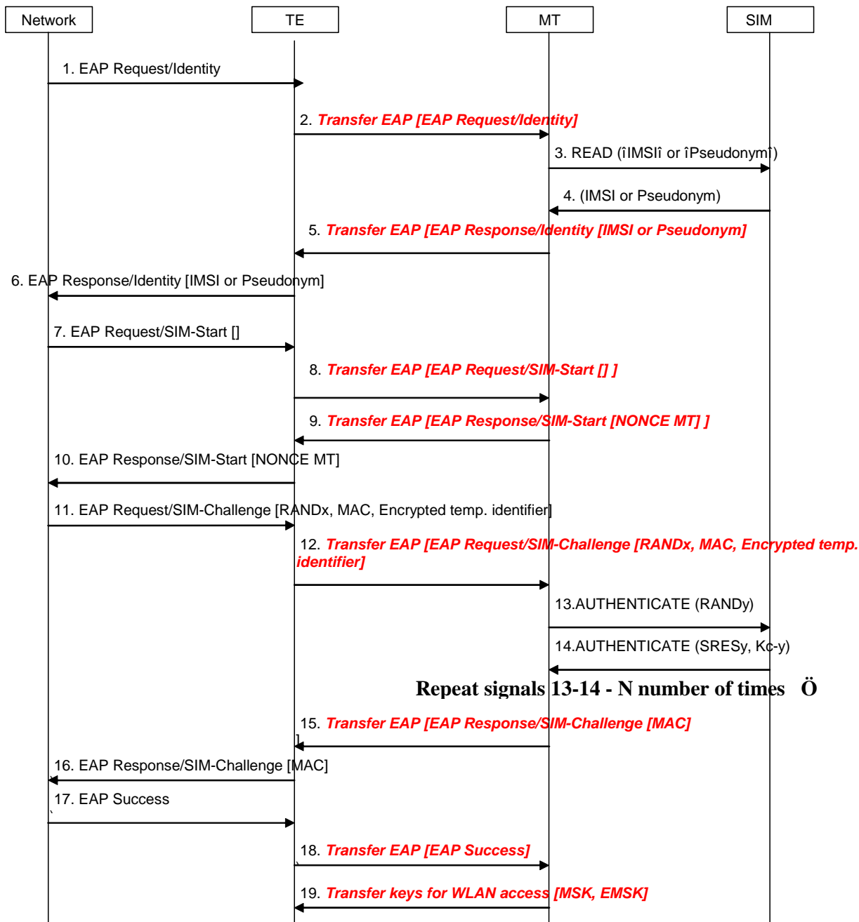
Figure 12: Full authentication with EAP SIM
