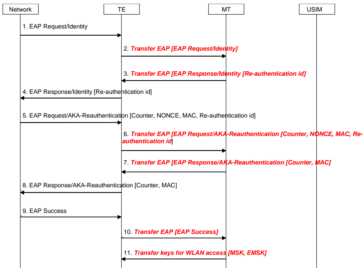
Figure 13: Fast re-authentication with EAP AKA
