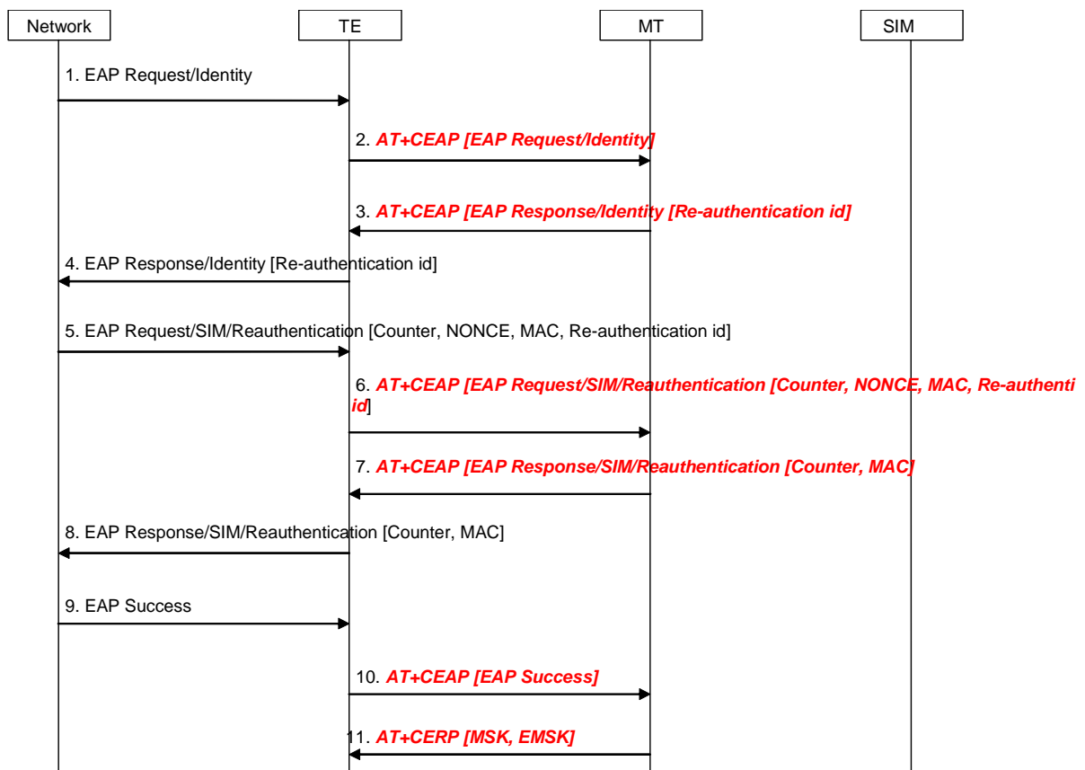
Figure 184: Fast re-authentication with EAP SIM
