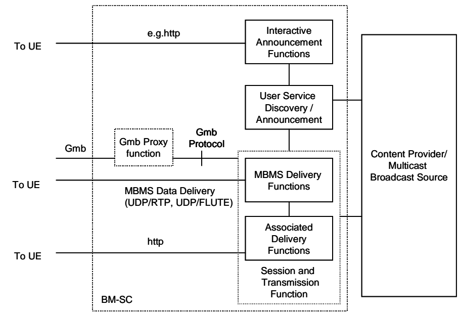
Figure 4: BM-SC sub-functional structure
