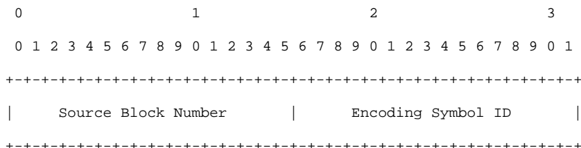
Figure 11: Example FEC Payload ID Format
