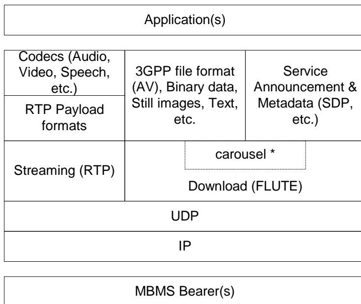
Figure 9: Protocol stack view of the MBMS User Services over MBMS bearer(s)
