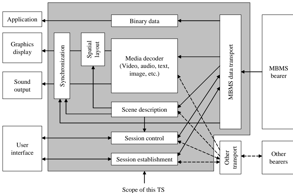
Figure 5: Functional components of an MBMS client
