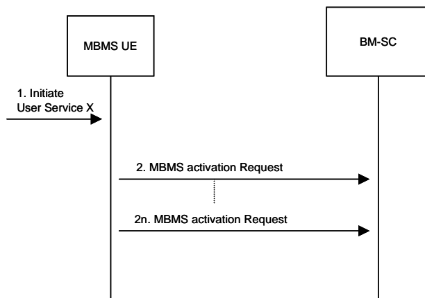
Figure 6: Initiation of an MBMS User Service
