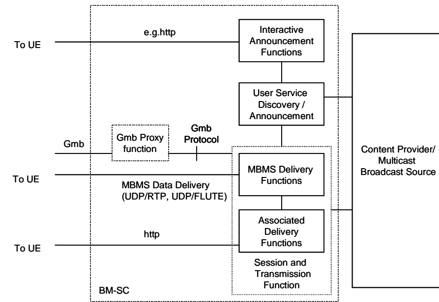
Figure 4: BM-SC sub-functional structure
