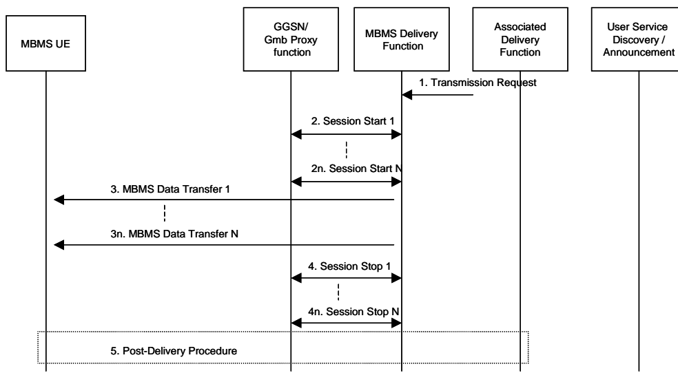
Figure 8: Procedure of MBMS Data Transfer
