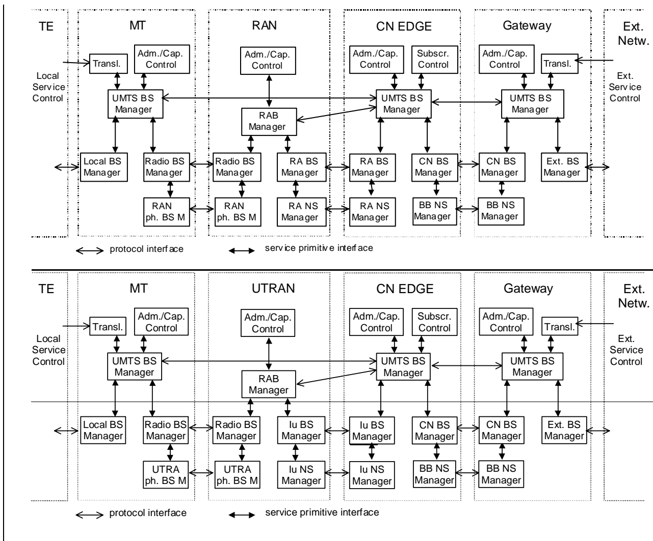
Figure 2: QoS management functions for UMTS bearer service in the control plane
