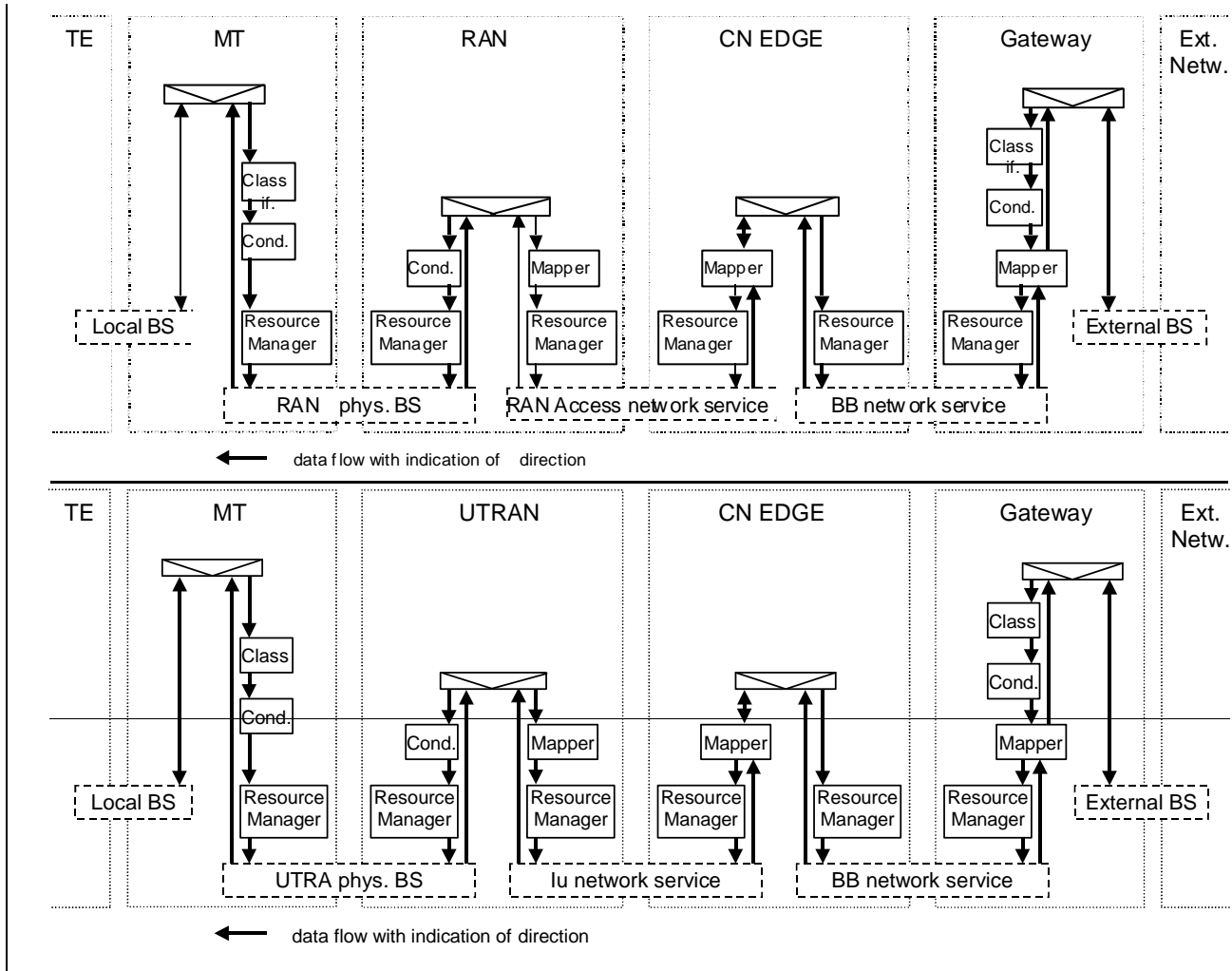
Figure 3: QoS management functions for the UMTS bearer service in the user plane
