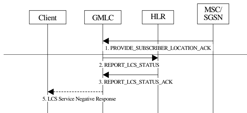
Figure 9.z: UE Presence Notification procedure
