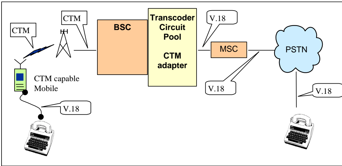
Figure B.1: CTM adaptor contained within a transcoder pool
