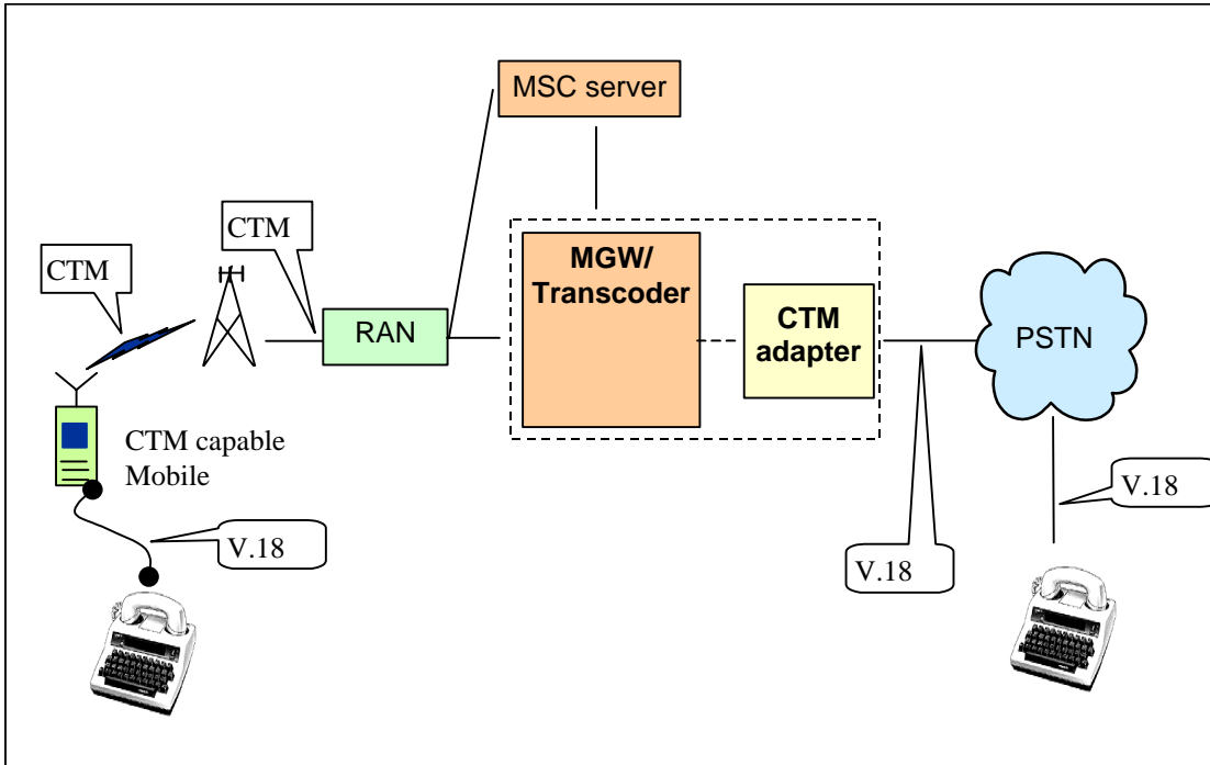
Figure B.2: Association of a CTM capable termination within the Media Gateway.
