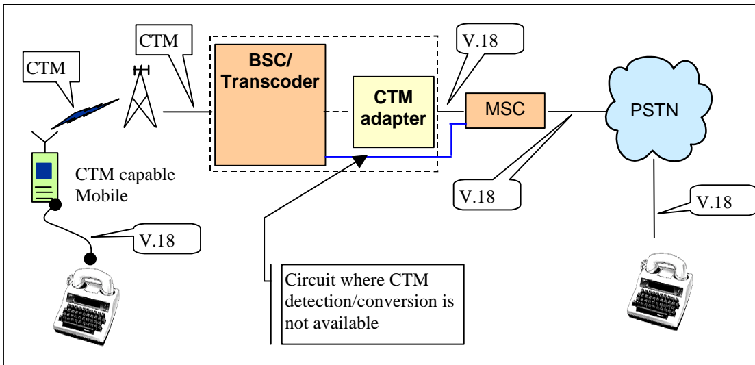
Figure B.2: CTM adaptor present on specific A-interface circuits
