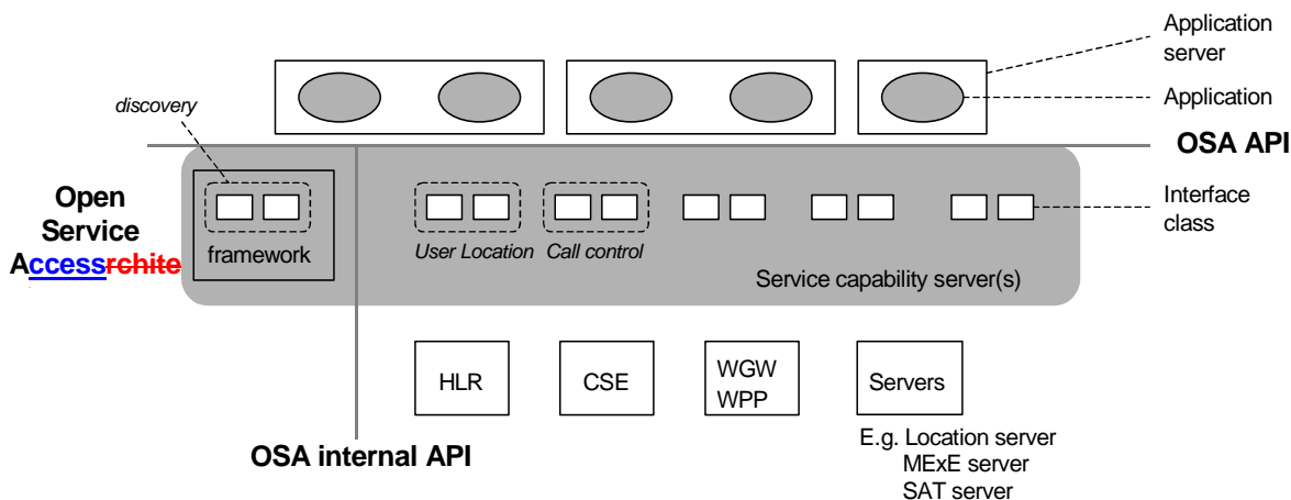
Figure 1: Overview of Open Service Architecture Open Service Access
