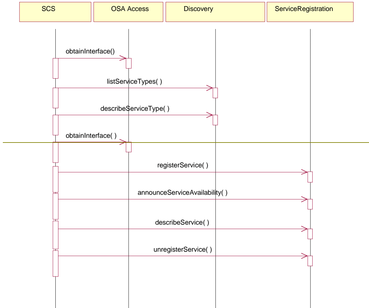
Figure 14: SCF Registration
