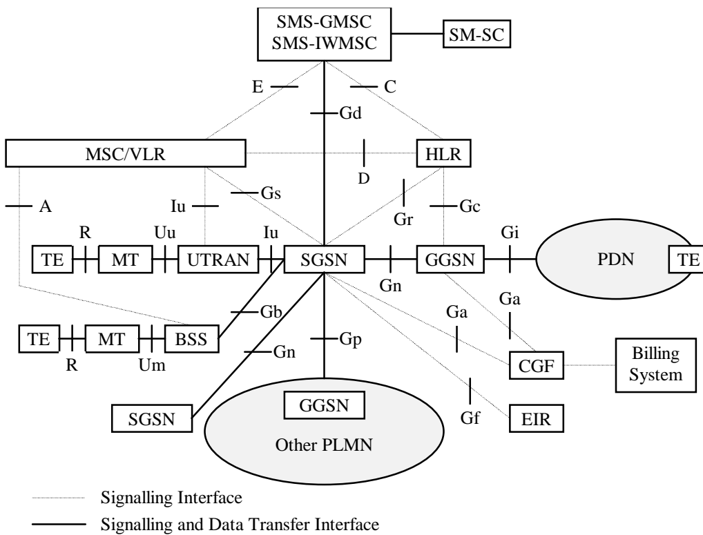
Figure 1: Overview of the GPRS Packet Domain Logical Architecture
