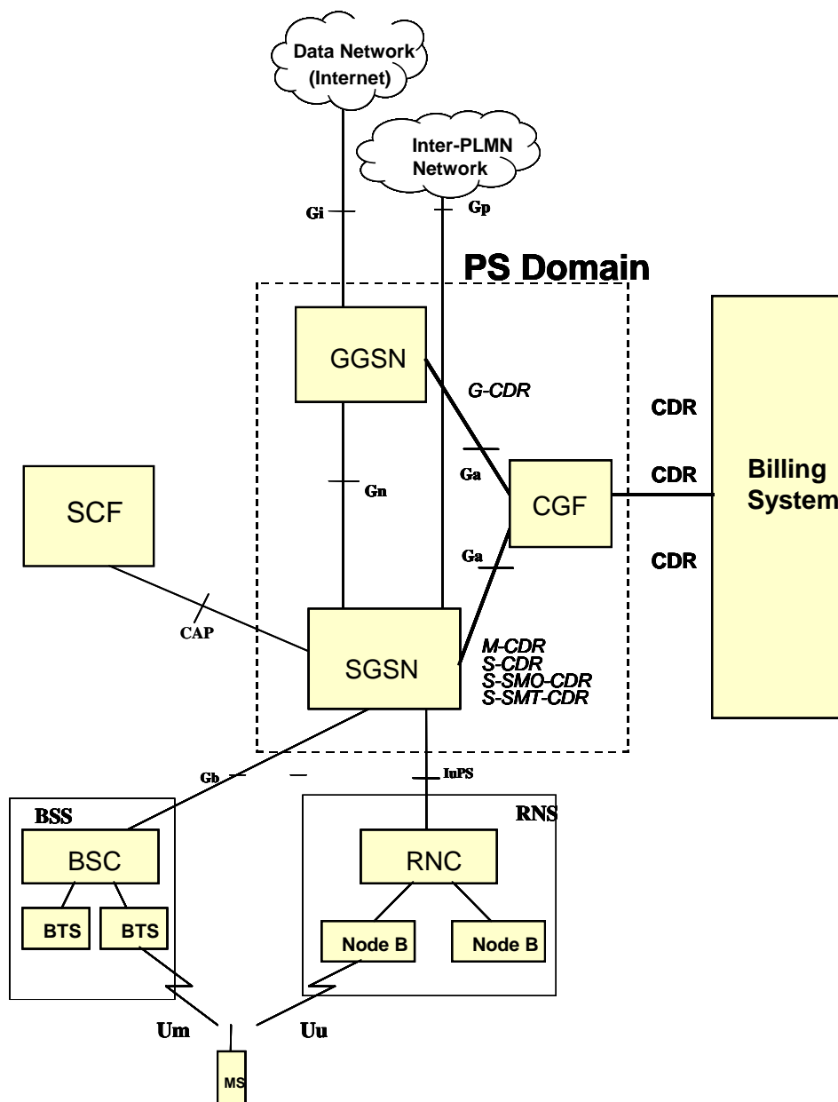
Figure 2: GPRS Packet Domain charging logical architecture
