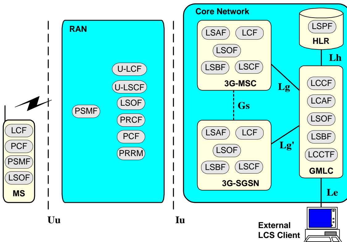
Figure 6.3, Generic LCS Logical Architecture
