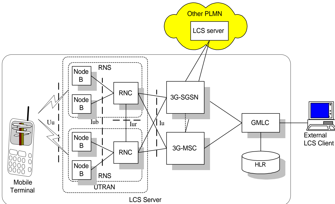
Figure 6.1, General arrangement of LCS in UMTS
