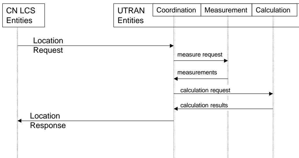
Figure 6.2, General sequence for LCS operation
