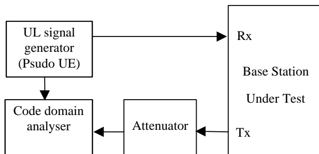
Fig. 6.4-1 Configuration for power control steps measurement
