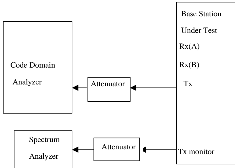
Fig. 6.4-4 Configuration for measurement
