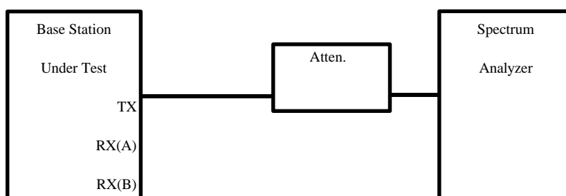
Fig. 6.5-1 Functional Setup for Transmission on/off Ratio Test.
