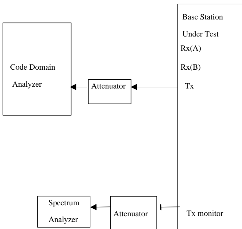
Fig. 6.4-3 Configuration for measurement
