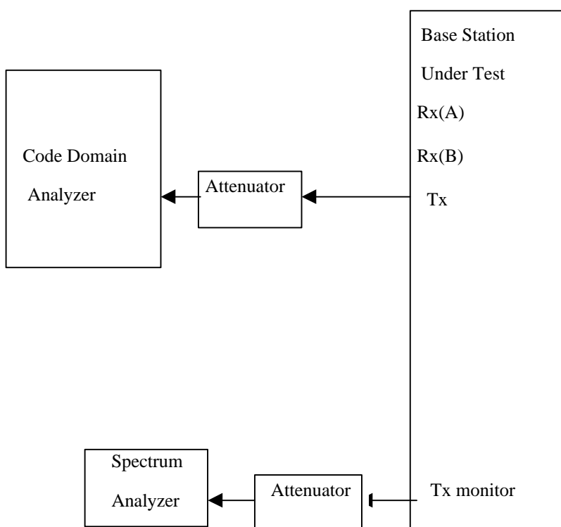
Fig. 6.4-2 Configuration for measurement
