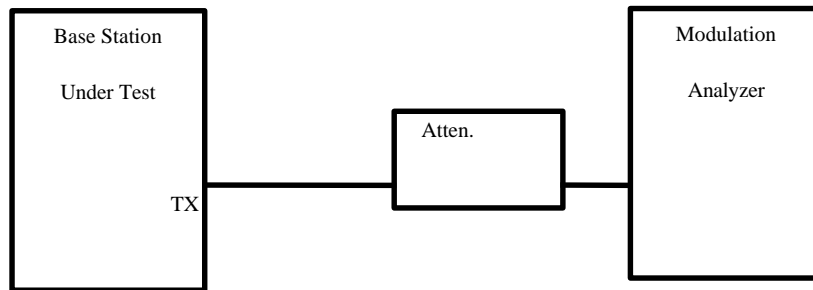
Fig. 6.8-1 Functional Setup for Modulation Accuracy Test.
