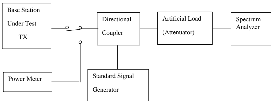
Fig. 6.7-1 Functional Setup for Base Station Intermodulation Spurious Response Testes
