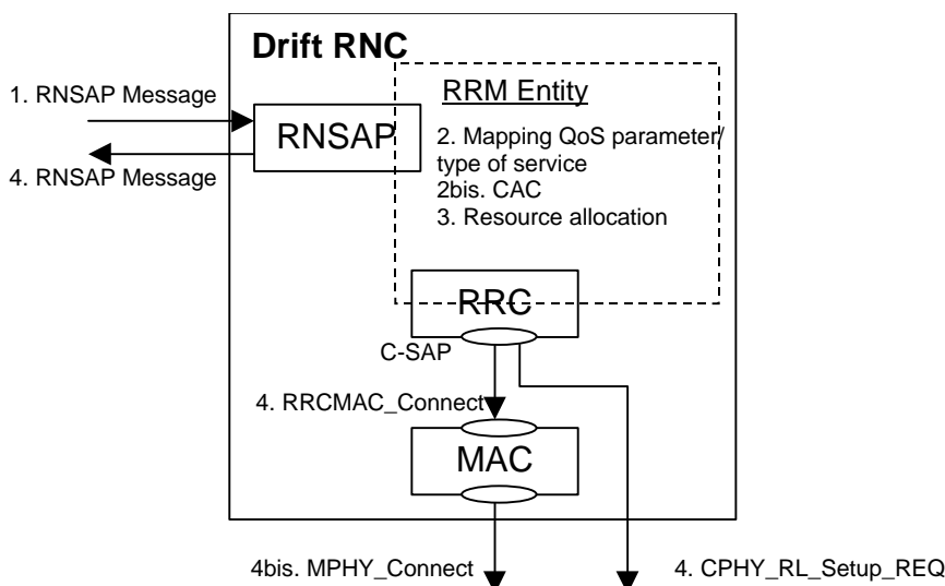
Figure 555: This model shows how standardized RNSAP and RRC layers are involved in the CAC process. The dashed box represents a proprietary entity.
