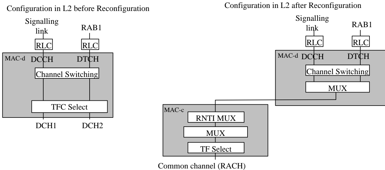
Figure 888 Configuration in the UTRAN UL before and after the Physical channel reconfiguration.
