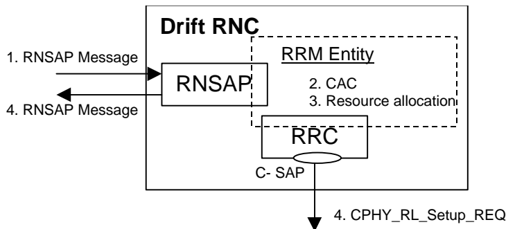
Figure 444: This model shows how standardized RNSAP and RRC layers are involved in the CAC process. The dashed box represents a proprietary entity.
