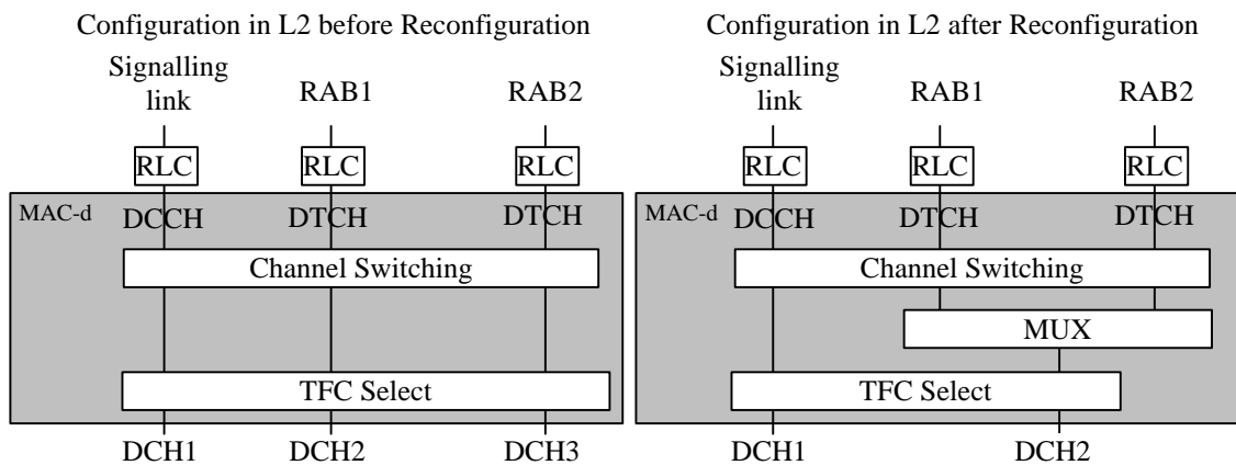
Figure 101010 Configuration in the UTRAN DL before and after the RAB reconfiguration.
