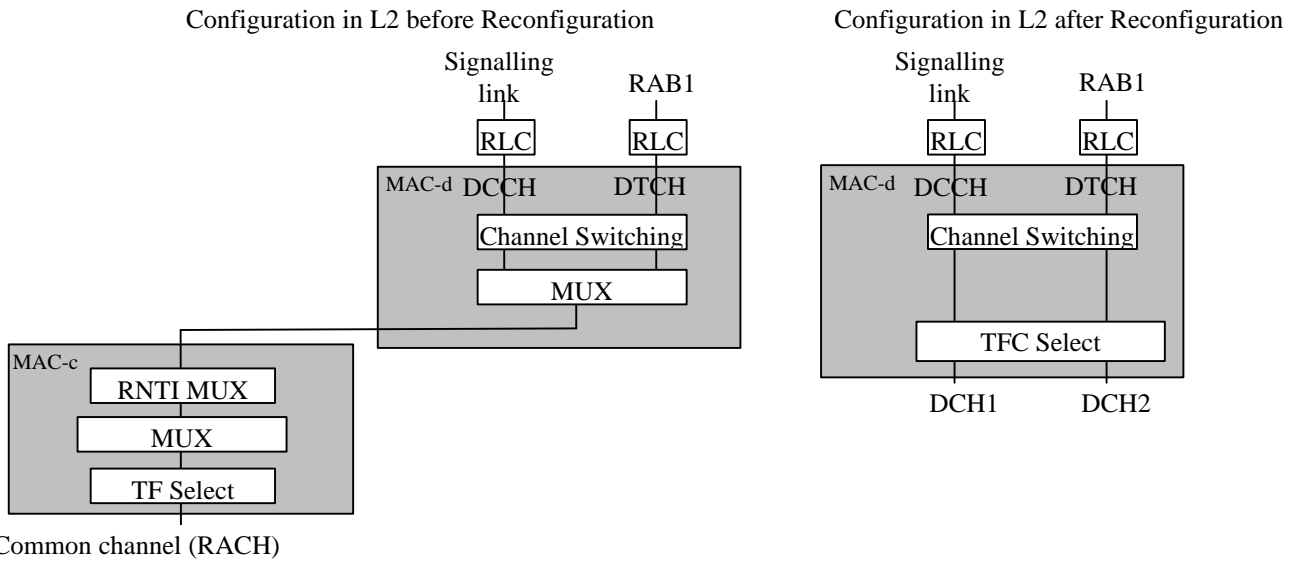
Figure 777 Configuration in the UTRAN UL before and after the Physical channel reconfiguration.
