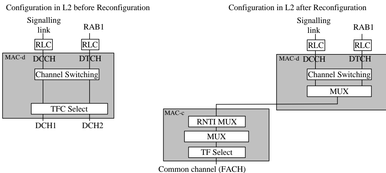
Figure 999 Configuration in the UTRAN DL before and after the Transport channel reconfiguration.
