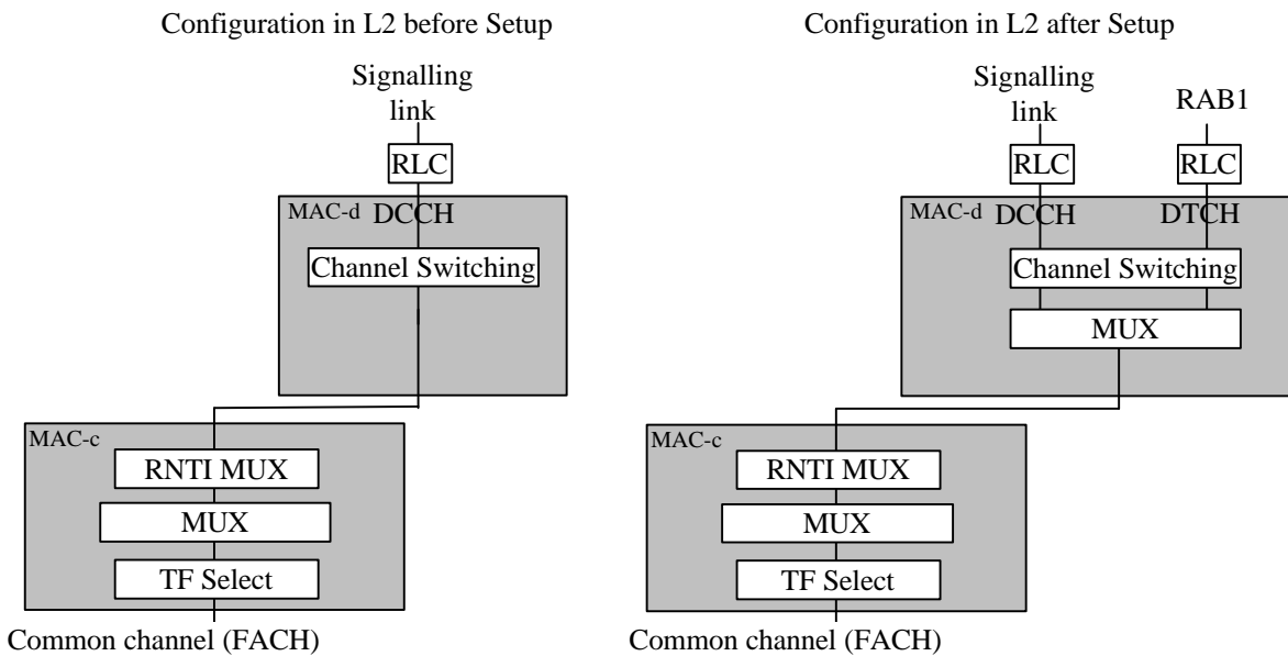
Figure 666 Configuration of L2 in the UTRAN DL before and after the RAB setup.
