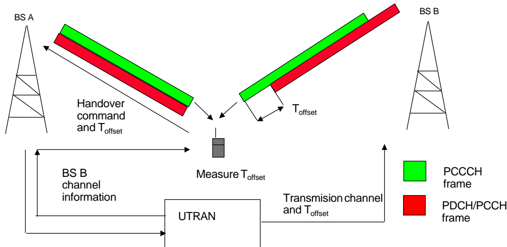
Figure 1. Making transmissions capable to be combined in the Rake receiver from timing point of view.
