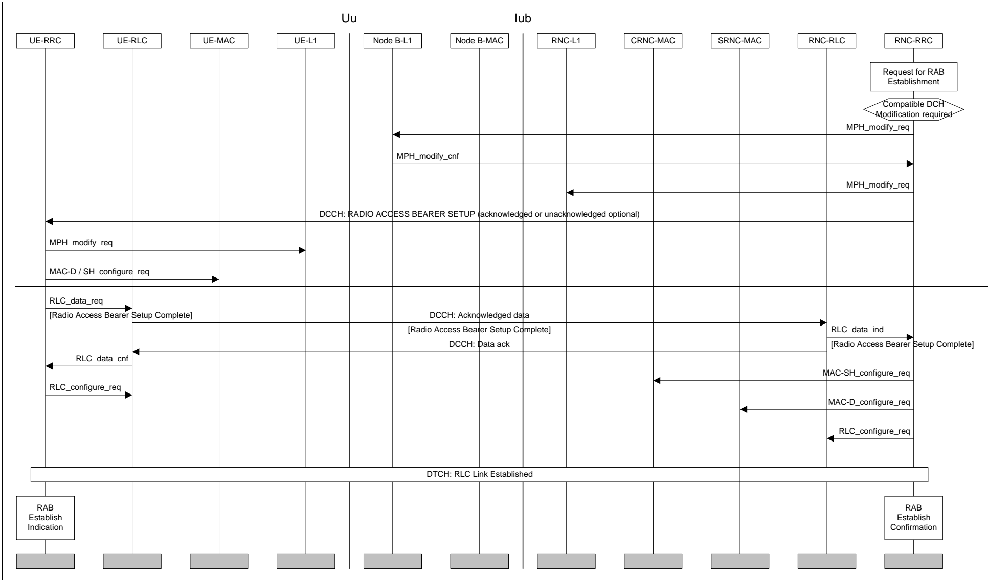
Figure 13: Radio Access Bearer Establishment with Unsynchronised Dedicated Physical Channel Modification
