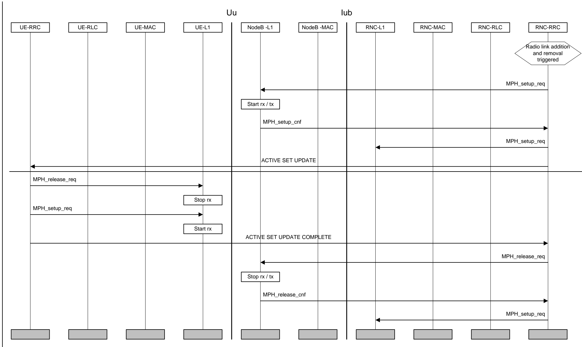
Figure 28: Combined Radio Link Addition And Removal
