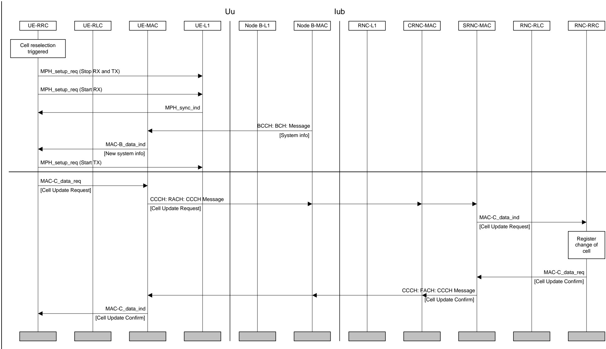
Figure 24: Cell update procedure
