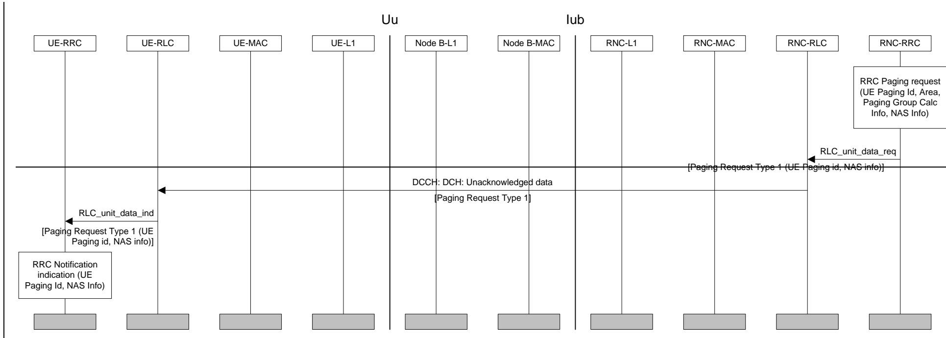
Figure 32. Example sequence of CN initiated paging request using DCCH
