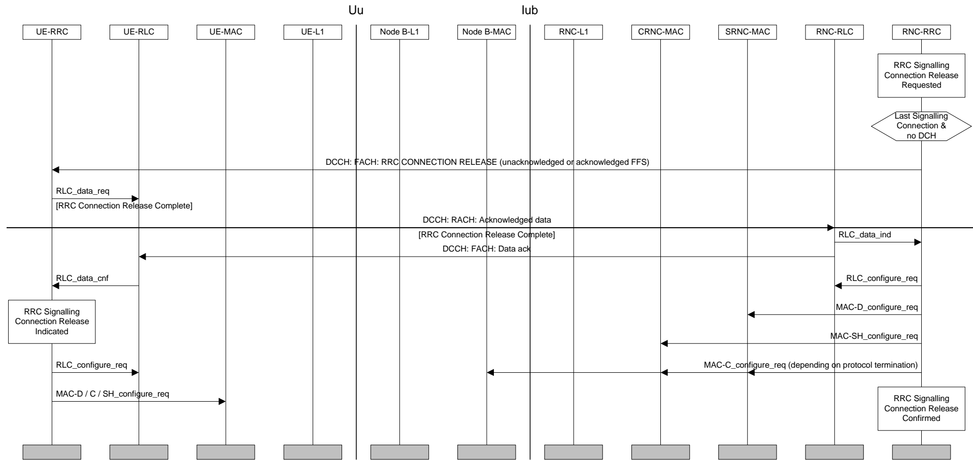
Figure 11: RRC Connection Release without Dedicated Physical Channel
