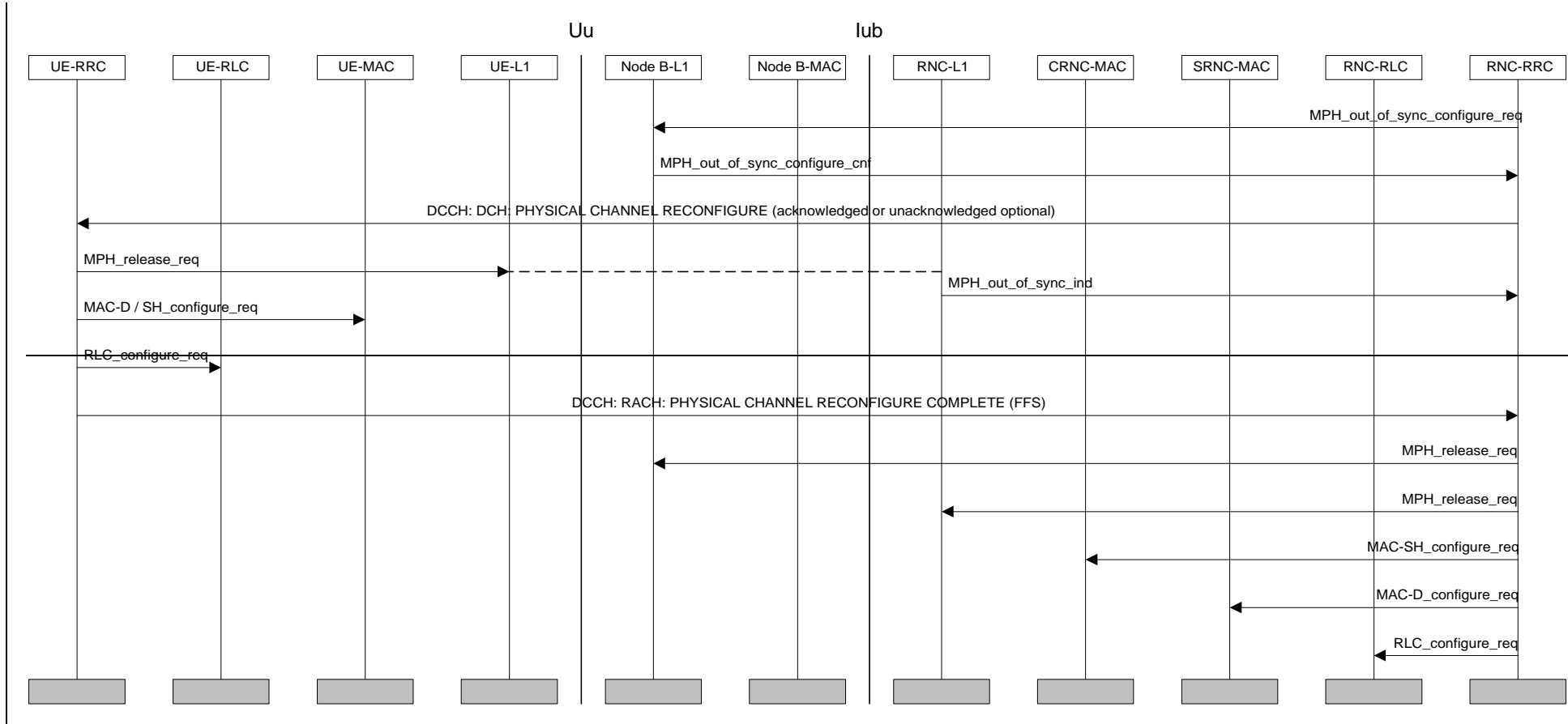
Figure 21: UE-terminated DCH Release
