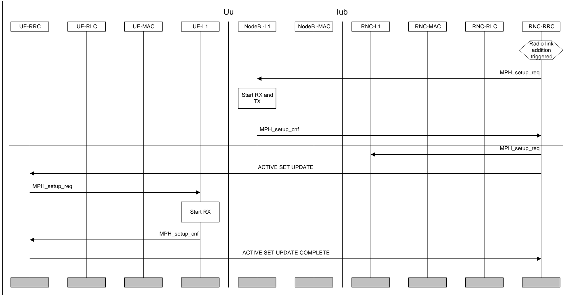
Figure 26: Radio Link Addition
