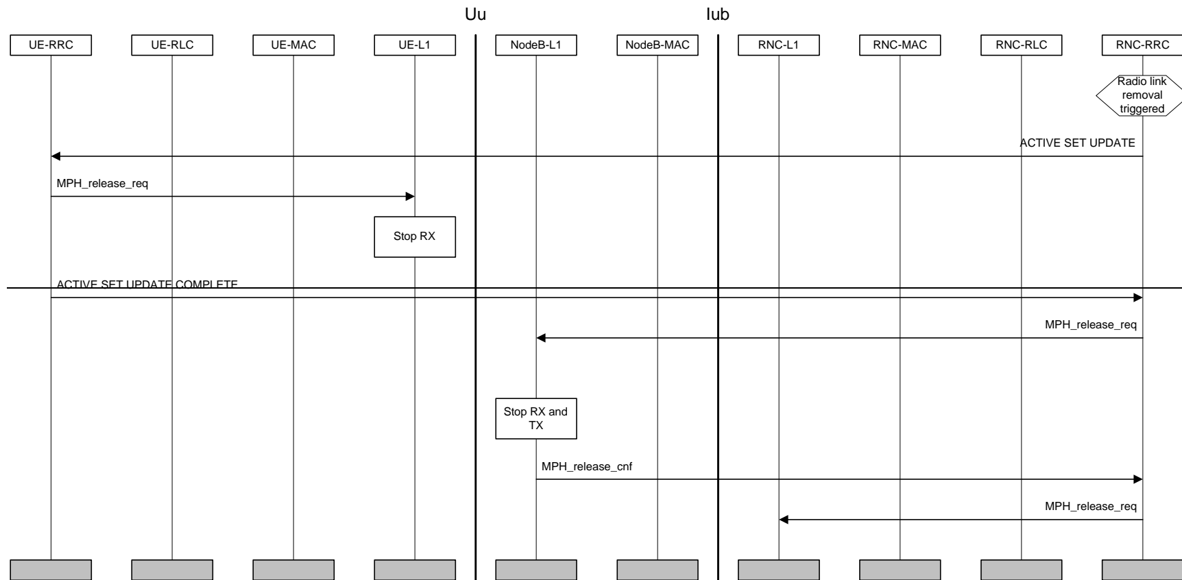
Figure 27: Radio link removal
