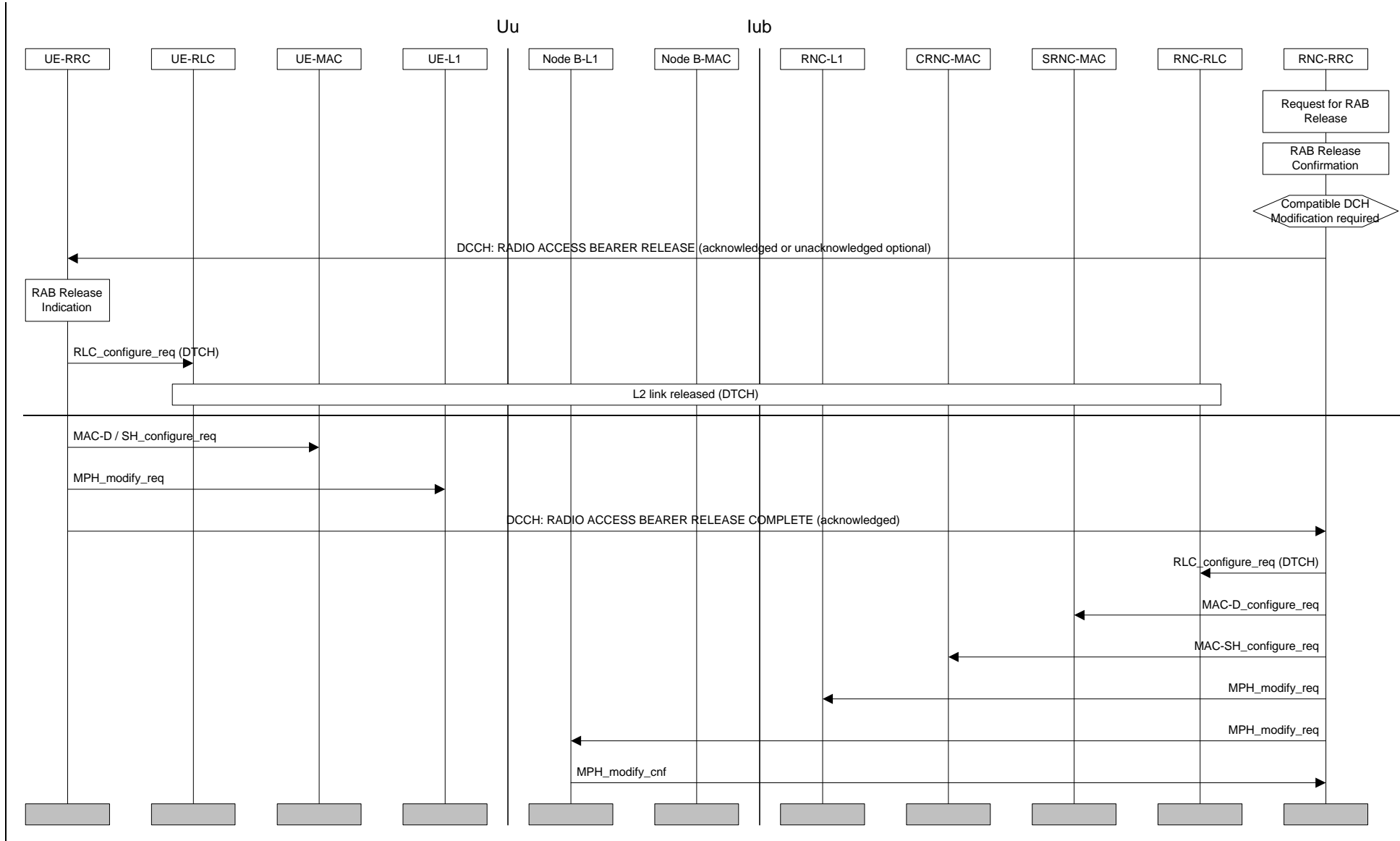
Figure 16: Radio Access Bearer Release with Unsynchronised Dedicated Physical Channel Modification
