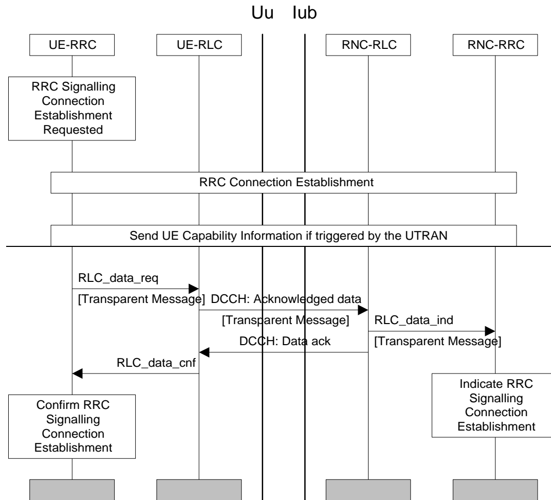
Figure 9. UE initiated Signalling Connection Establishment
