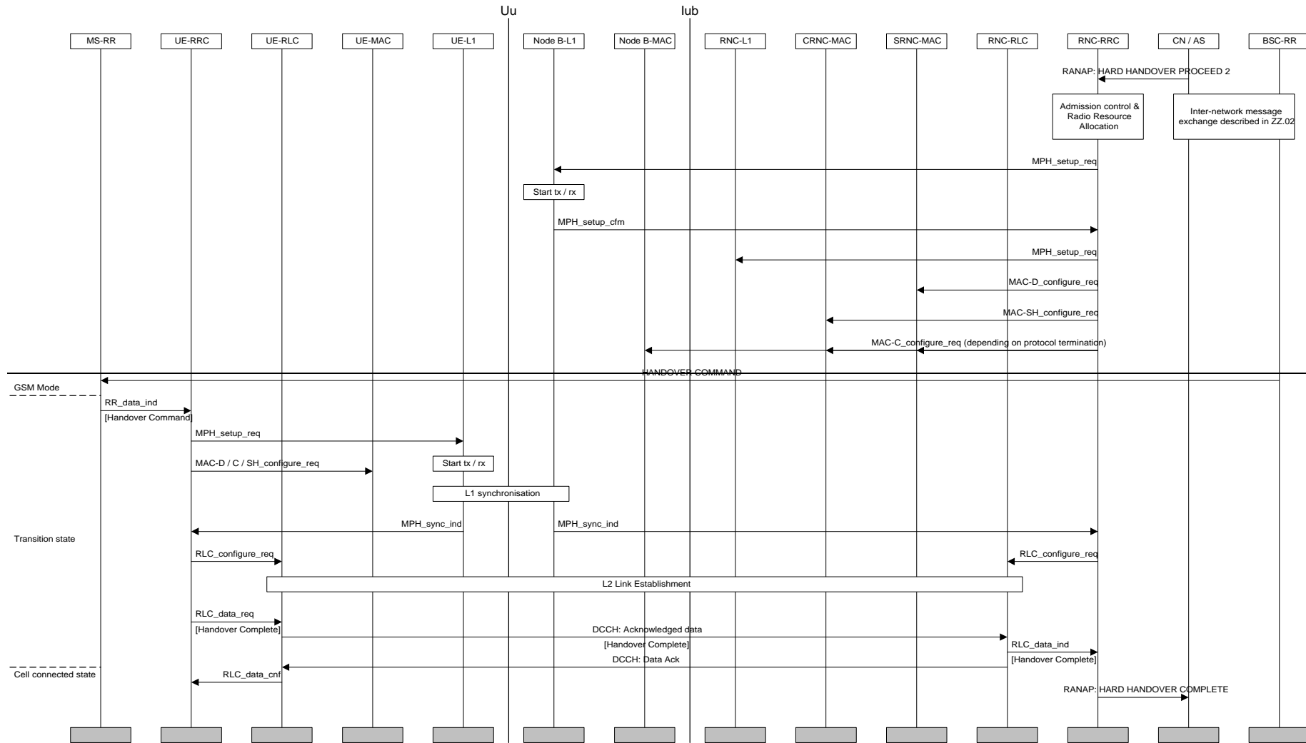
Figure 31: GSM to UMTS inter-system handover
