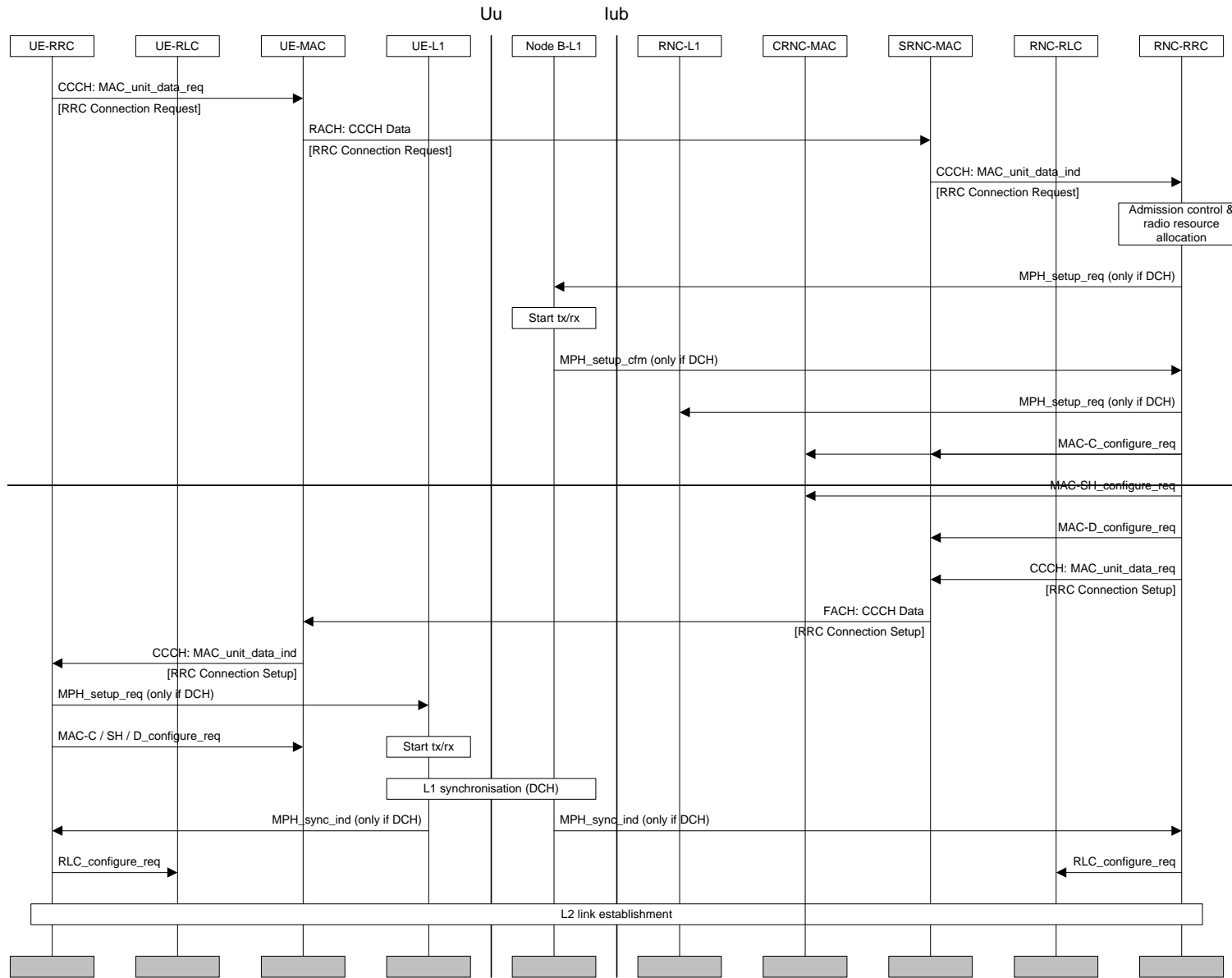
Figure 7. RRC connection establishment with common channel termination case A
