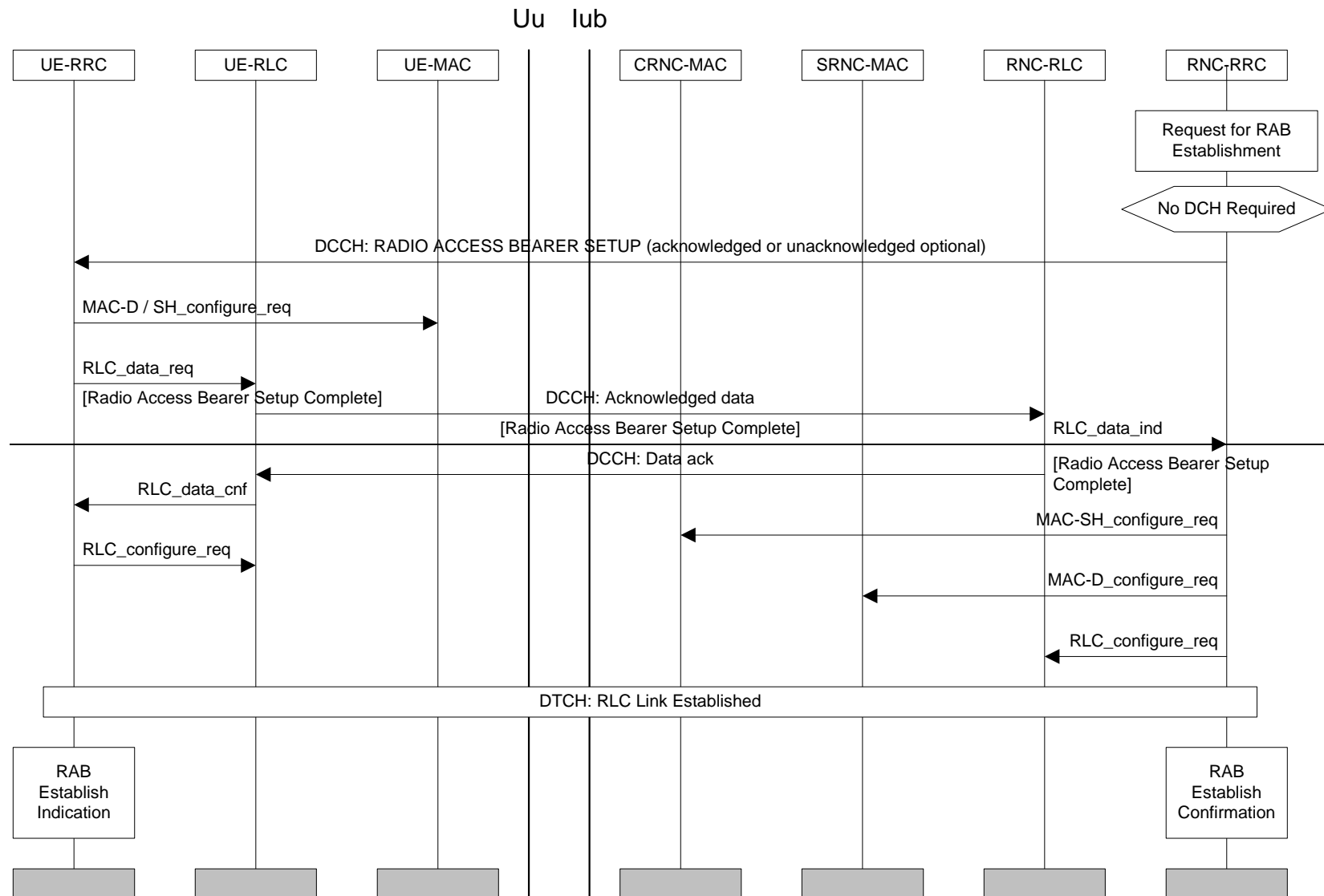
Figure 15: Radio Access Bearer Establishment without Dedicated Physical Channel
