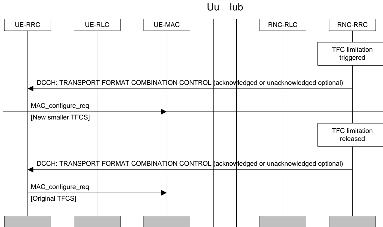
Figure 22: Transport Format Combination Limitation
