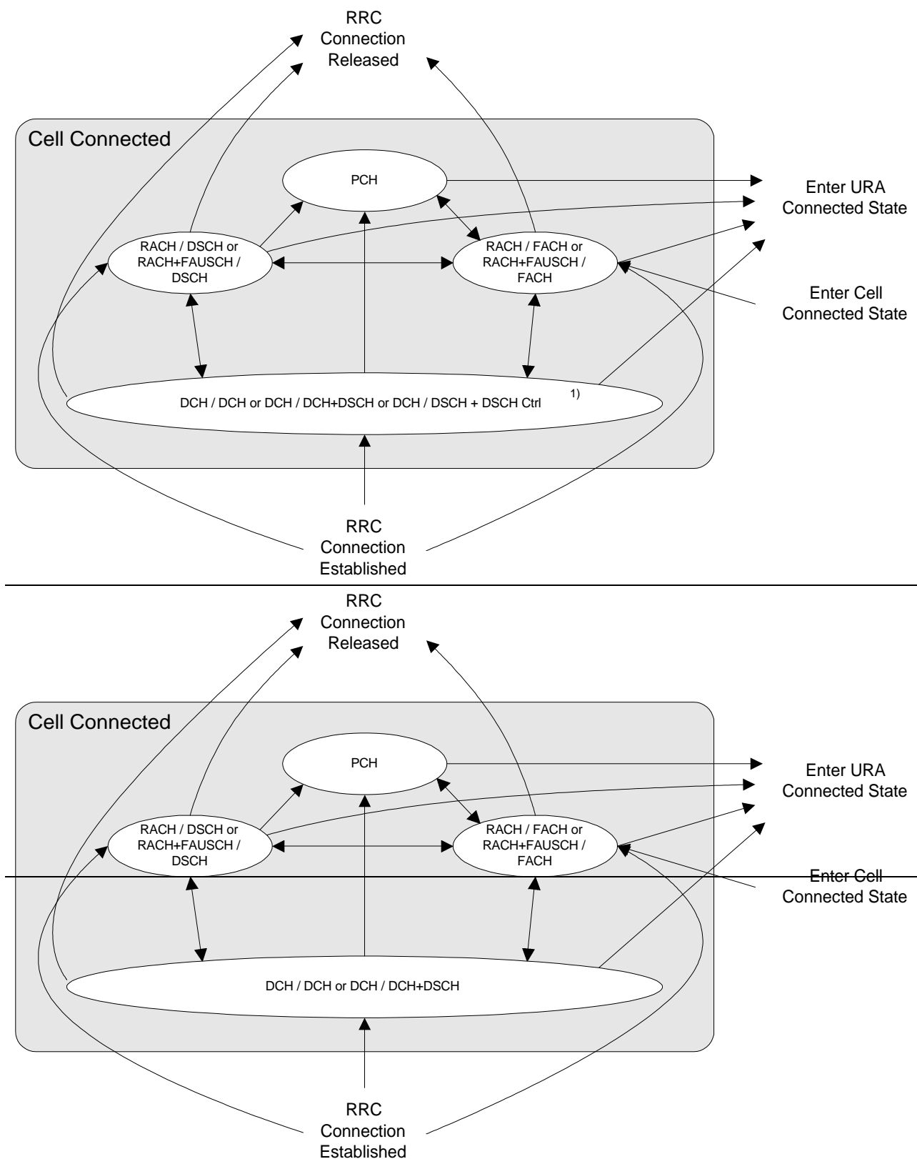
Figure 4: Substates within Cell Connected State
