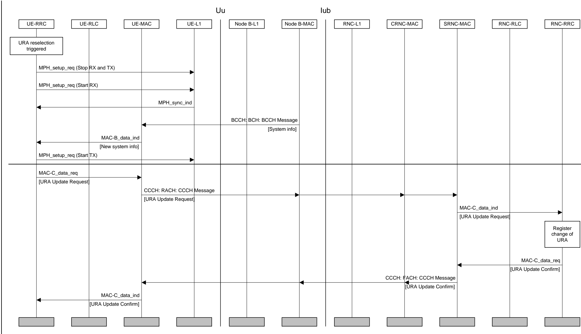
Figure 25: URA update procedure
