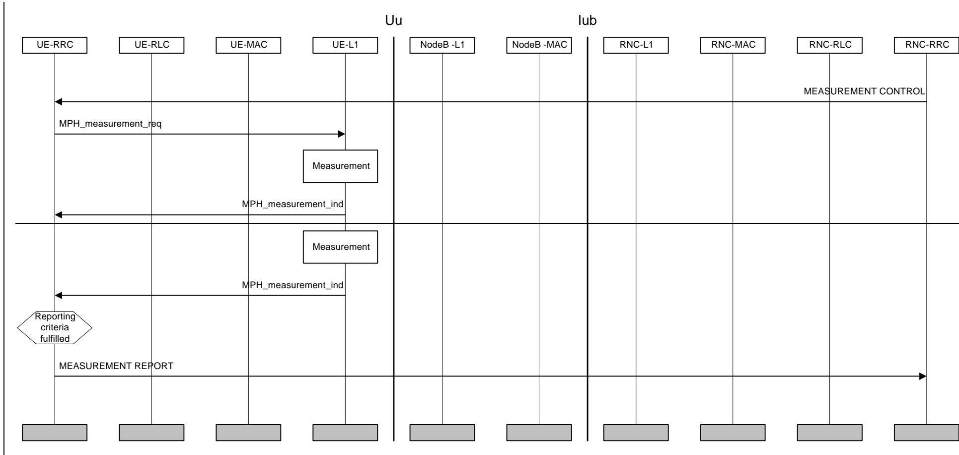
Figure 23: Handover measurement reporting
