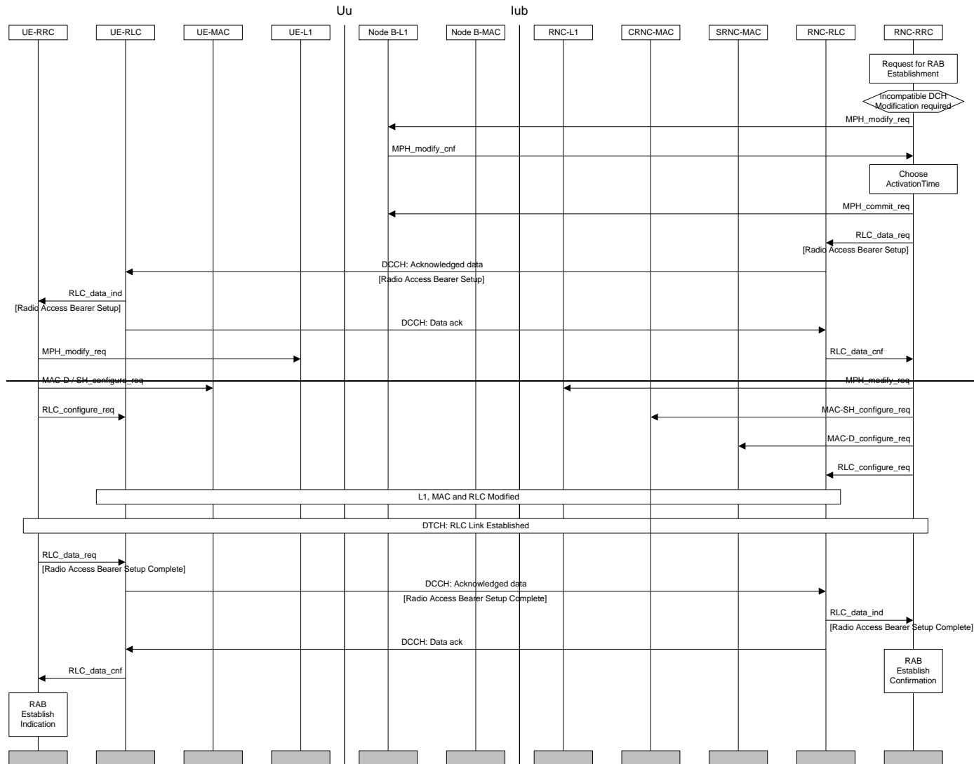
Figure 14: Radio Access Bearer Establishment with Synchronised Dedicated Physical Channel Modification
