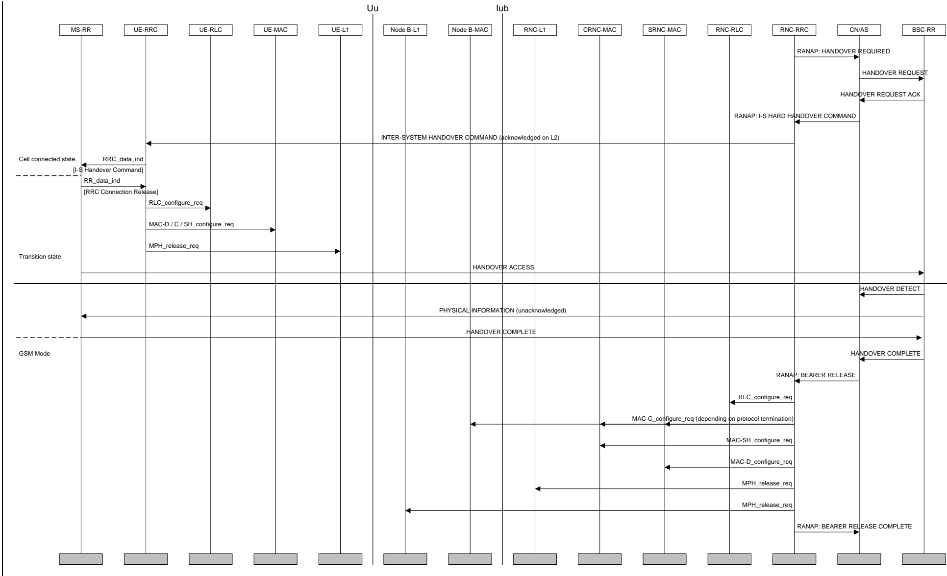
Figure 2. UMTS to GSM inter-system handover.
