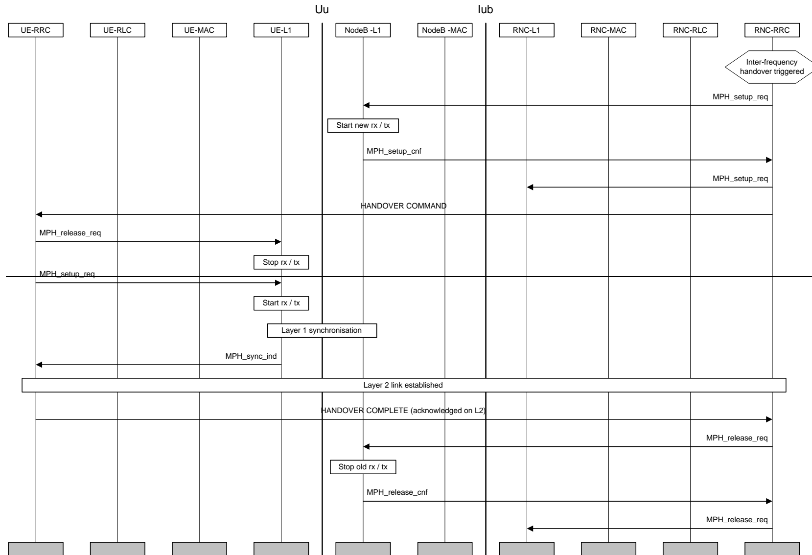
Figure 29: Hard handover
