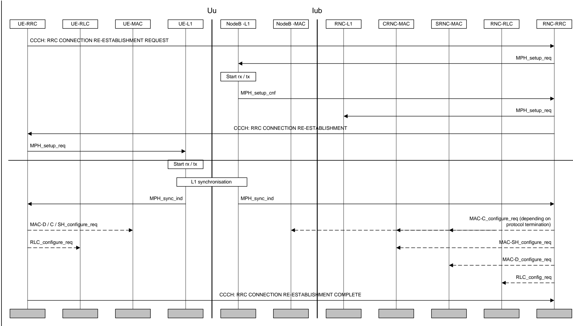
Figure 30: RRC connection re-establishment
