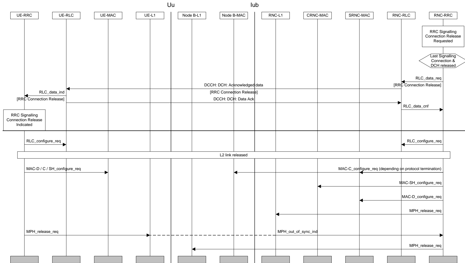
Figure 10. RRC Connection Release from Dedicated Physical Channel
