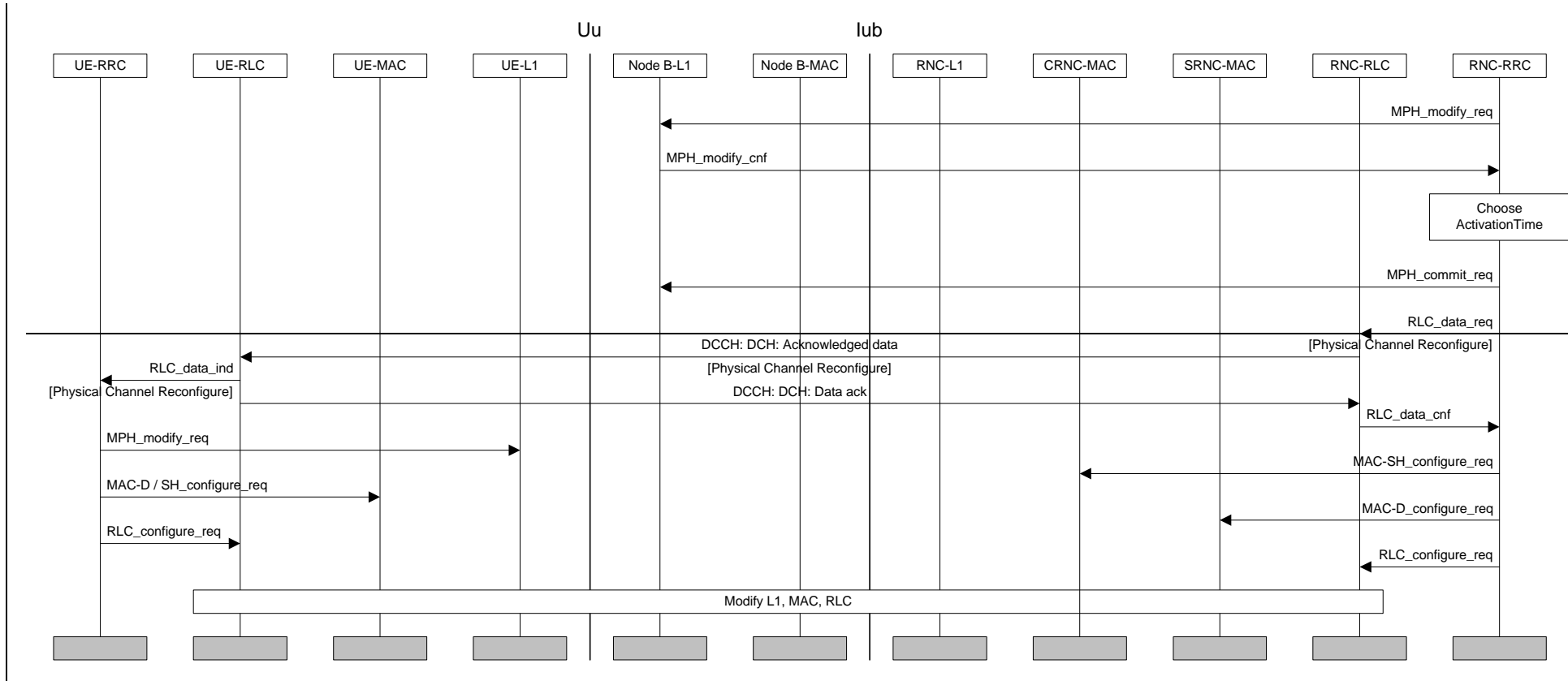
Figure 20: UE-terminated synchronised DCH Modify
