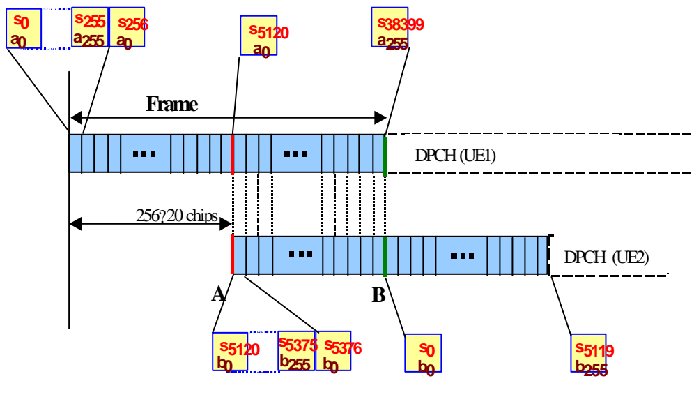
Figure 4.32 Timing at Node B and usage of scrambling and orthogonal codes in case of two UEs (a,b : channelisation codes, s : scrambling code, SF = 256)
