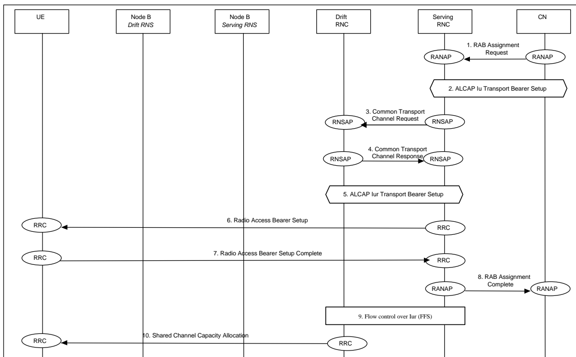
Radio Access Bearer Establishment - DSCH Establishment in RACH/FACH State
