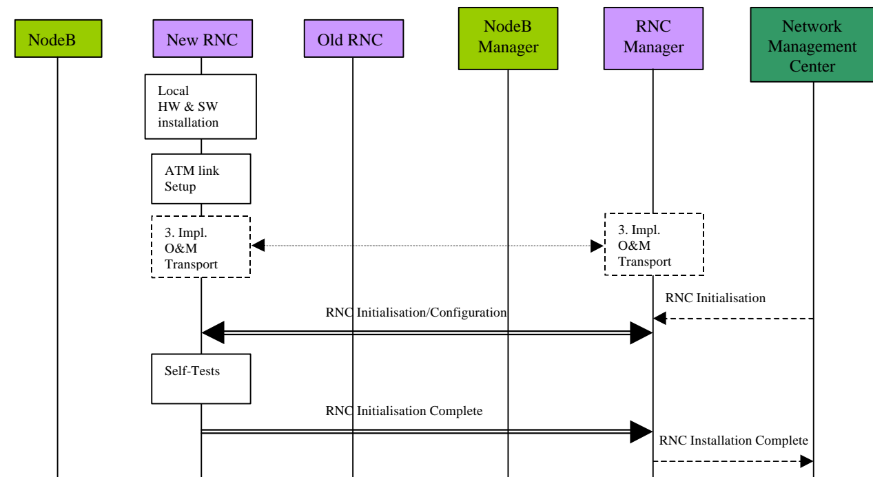
Figure 10.1.7.1.1 : RNC Installation
