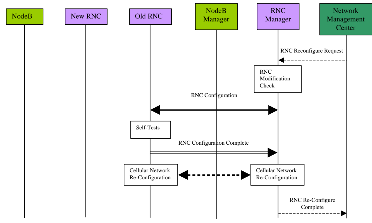
Figure 10.1.7.2.1 : RNC Re-configuration
