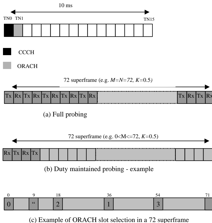
Figure 4: ORACH Superframe selection
