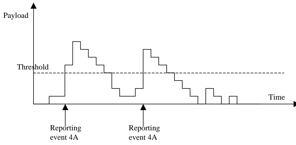
Figure 1: Figure 5246 Event triggered report when RLC buffer payload exceeds a certain threshold.
