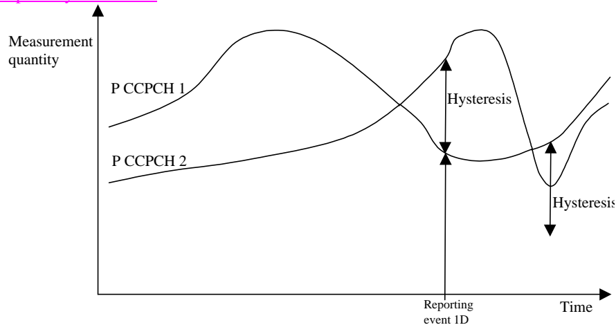
Figure 7:Figure 4442 Hysteresis limits the amount of measurement reports.
