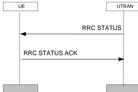
Figure 3432: RRC status procedure
