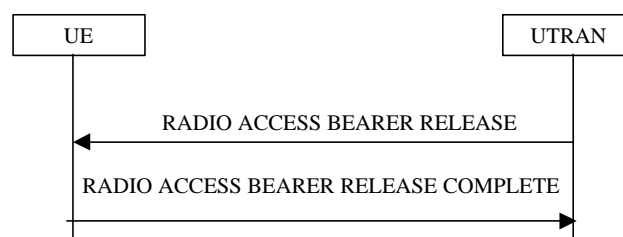
Figure 1411) Radio Access Bearer Release Procedure
