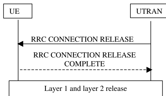
Figure 118) RRC Connection release procedure
