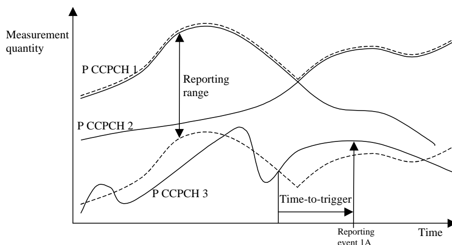
Figure 8:Figure 4643 Time-to-trigger limits the amount of measurement reports.
