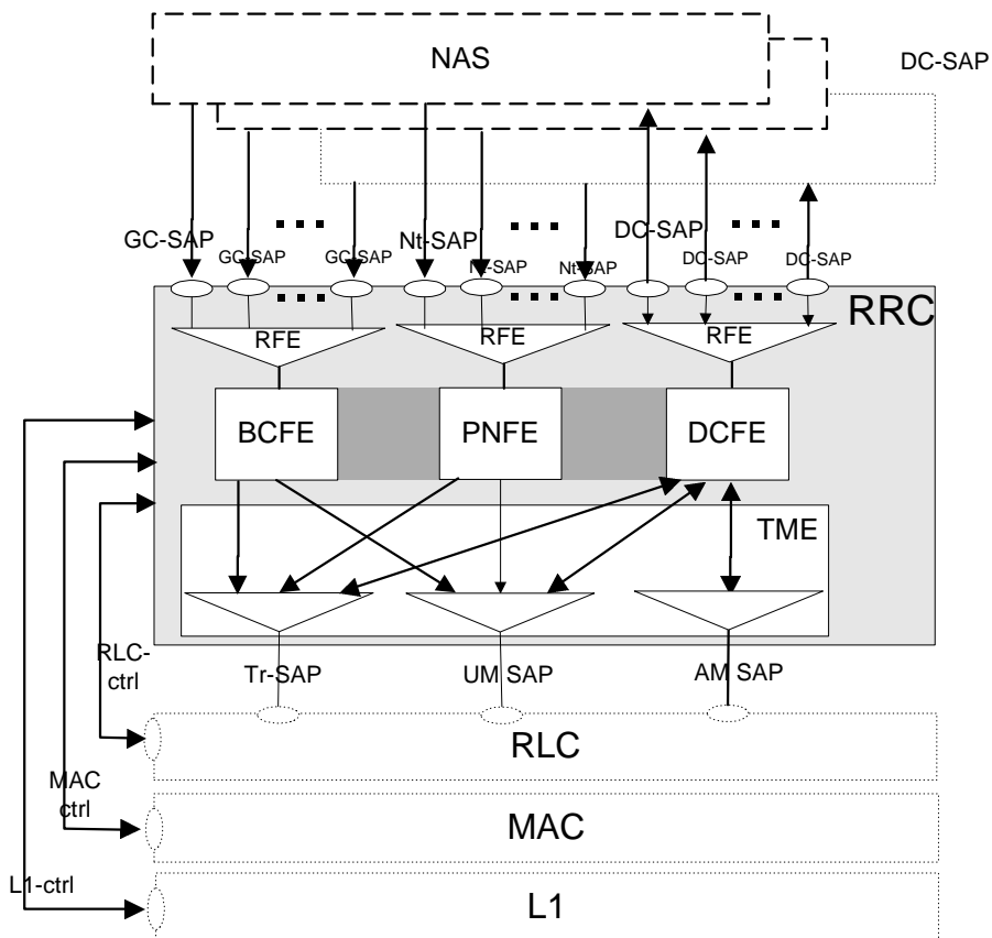
Figure 32) UTRAN side RRC model
