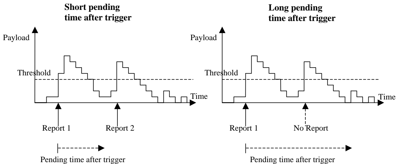
Figure 2- Figure 5347 Pending time after trigger limits the amount of consecutive measurement reports.
