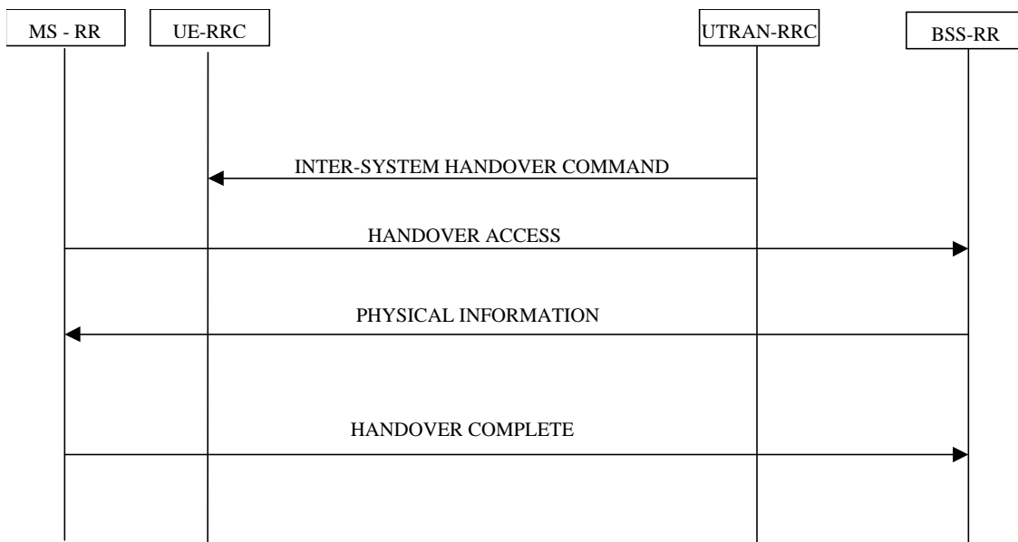
Figure 2220) Inter system hard hand-over (UTRAN to GSM/BSS), PSTN/ISDN services, successful case
