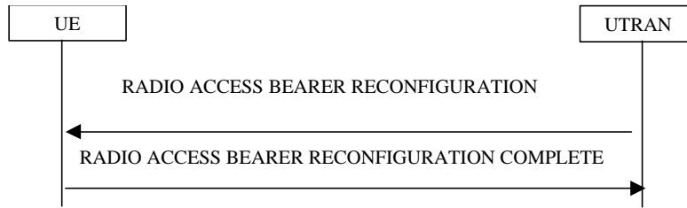
Figure 1512) Radio Access Bearer and signalling link Reconfiguration Procedure
