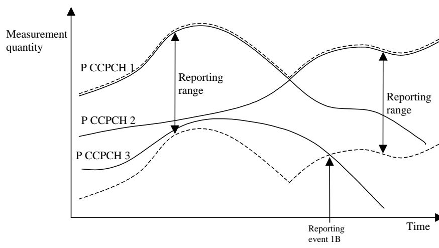
Figure 2: Figure 3735 Event-triggered report when a primary CCPCH leaves the reporting range.
