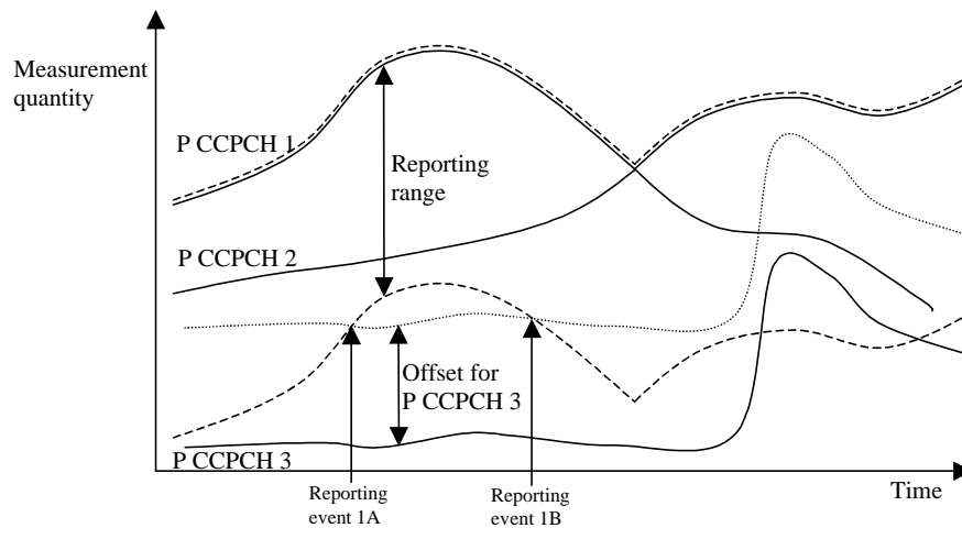
Figure 9: Figure 4844 A positive offset is applied to primary CCPCH 3 before event evaluation in the UE.
