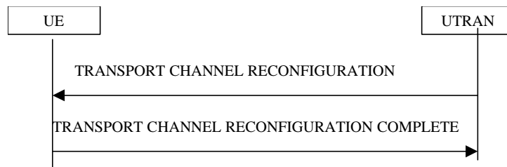
Figure 1613) Procedure for transport channel reconfiguration
