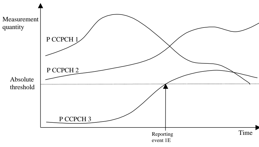
Figure 4038 Event-triggered report when a Primary CCPCH becomes better than an absolute threshold.
