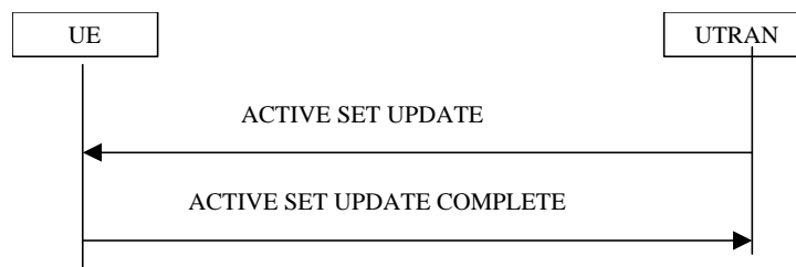
Figure 1917) Procedure for modifying the active set when in soft hand-over
