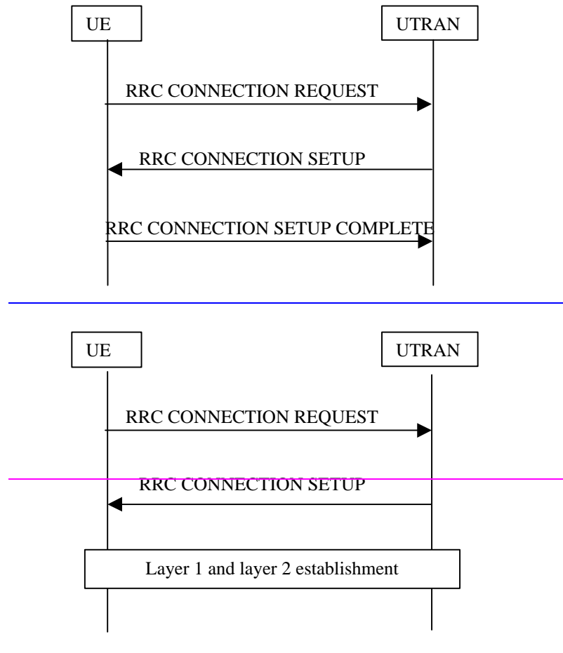
Figure 107) Procedure for RRC connection establishment
