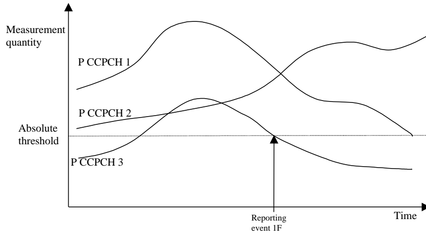
Figure 4139 Event-triggered report when a Primary CCPCH becomes worse than an absolute threshold.
