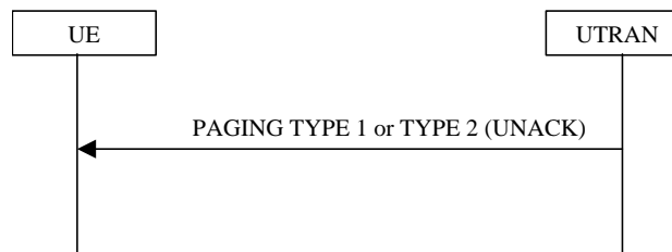
Figure 2624) Core network originated paging procedure in connected mode
