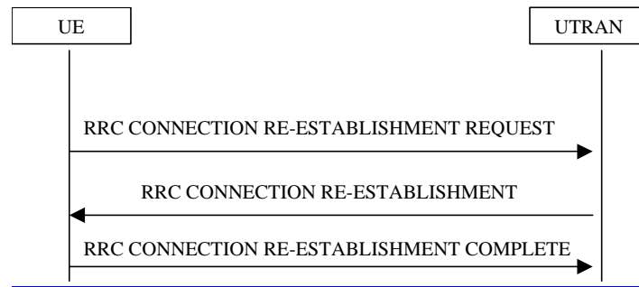
Figure 129) RRC Connection re-establishment
