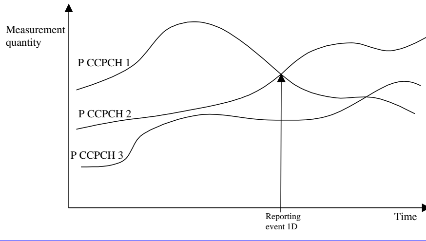
Figure 3- Figure 3937 A primary CCPCH becomes better than the previously best primary CCPCH.
