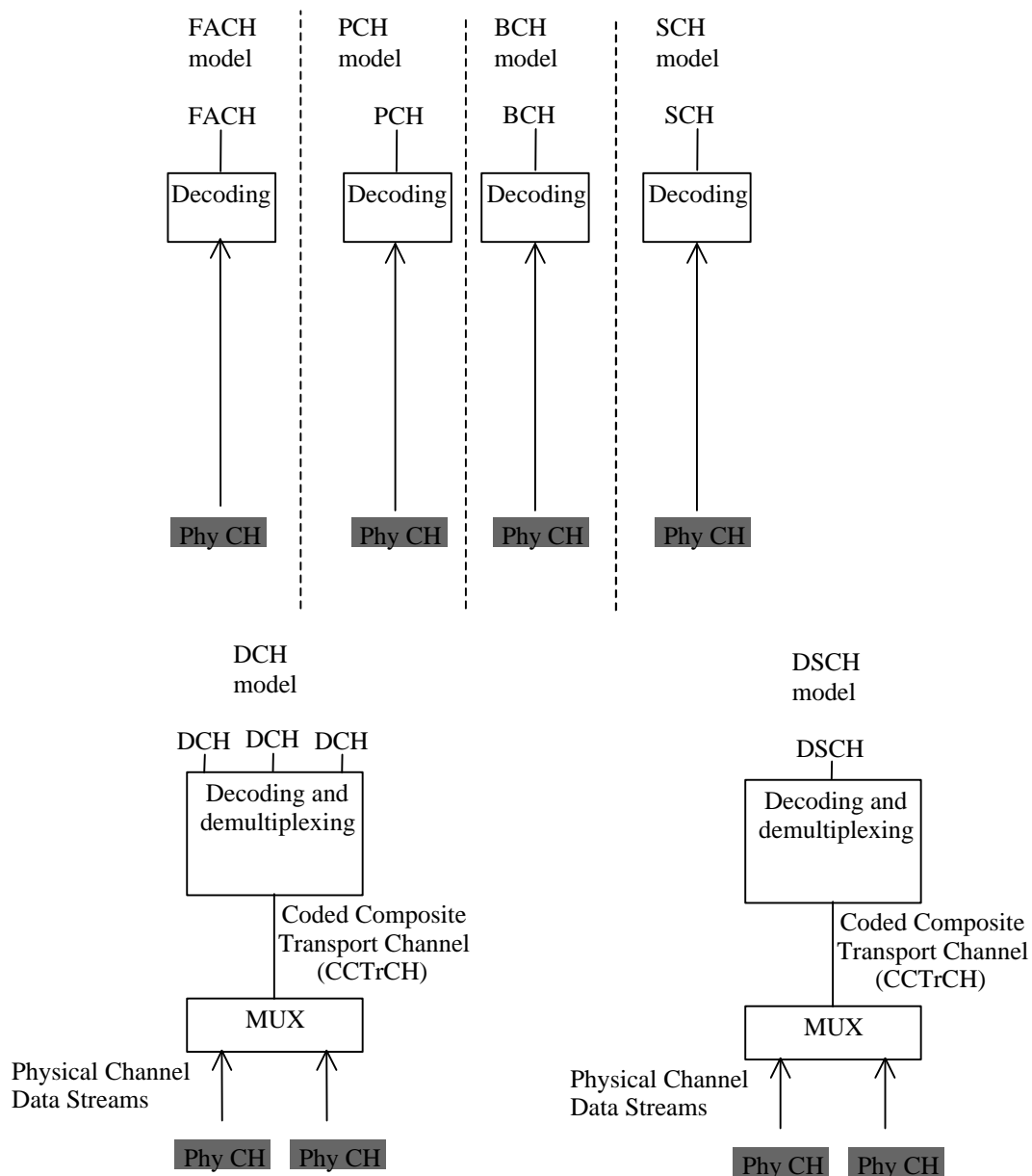
Figure 44: Model of the UE's physical layer – downlink TDD mode
