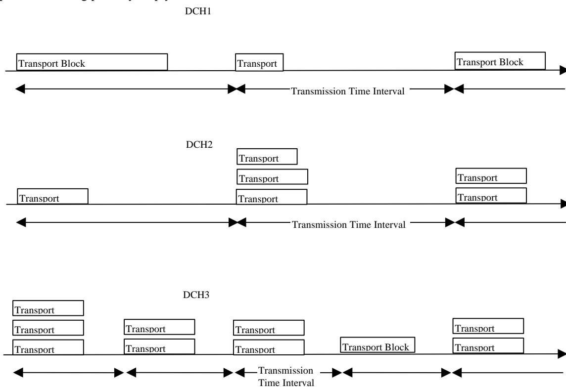
Figure 66. Exchange of data between MAC and L1
