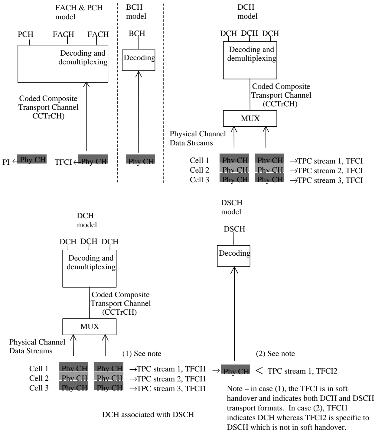
Figure 33: Model of the UE's physical layer – downlink FDD mode
