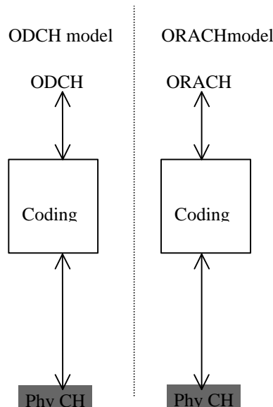
Figure 55 : Model of the UE's physical layer - relay link TDD mode.
