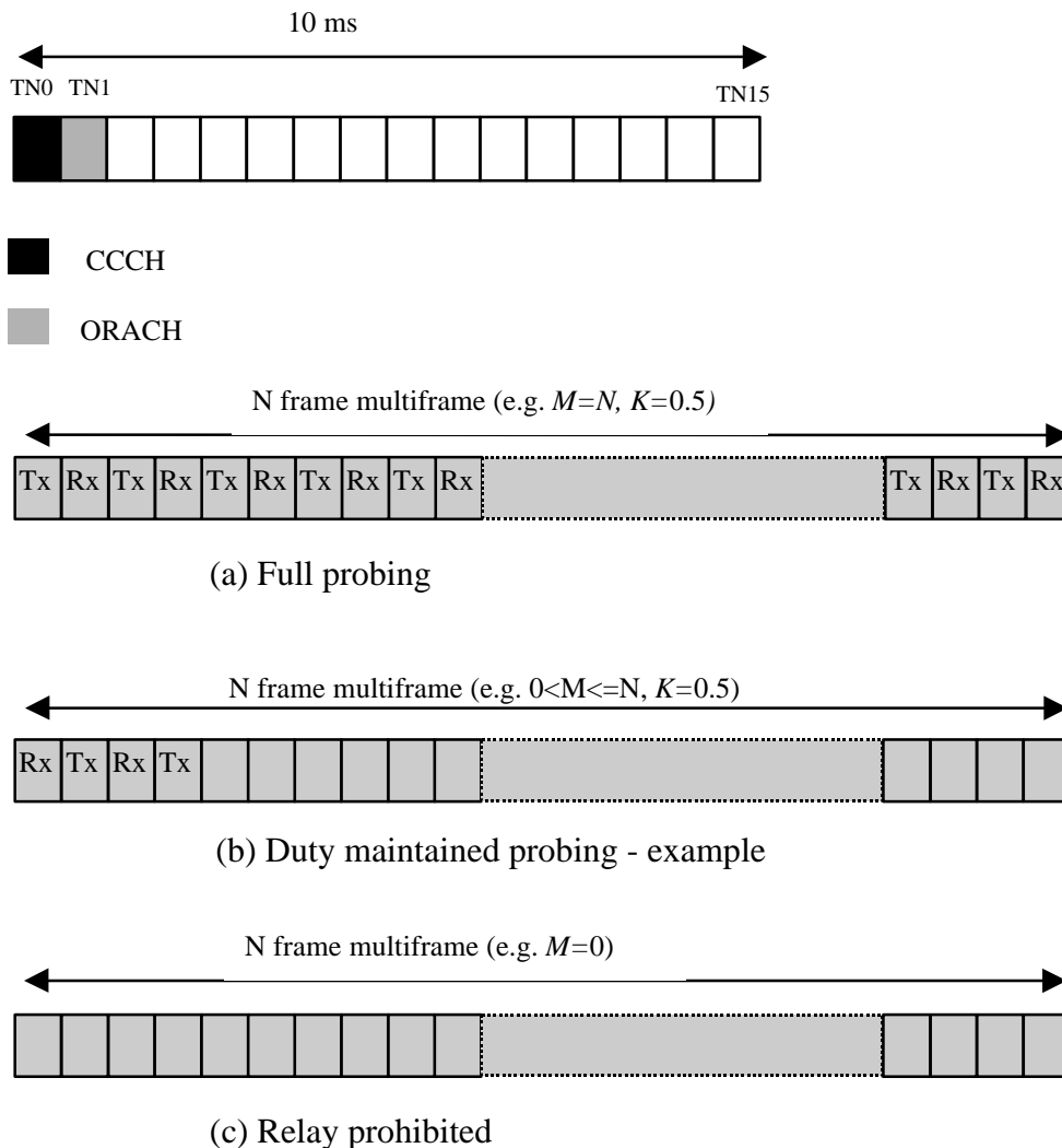
Figure 22. Probing state machines and mechanism.
