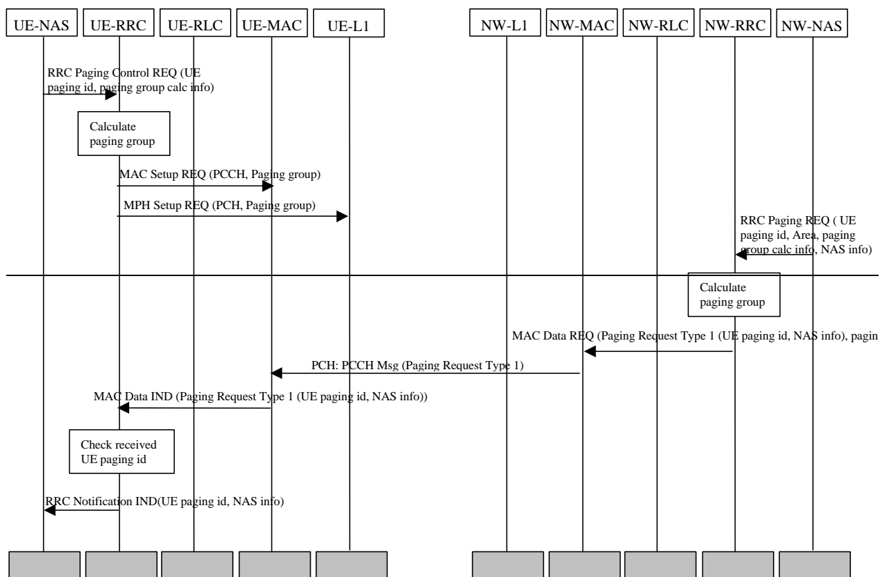
Figure 7. Example sequence of CN initiated paging request in idle mode.
