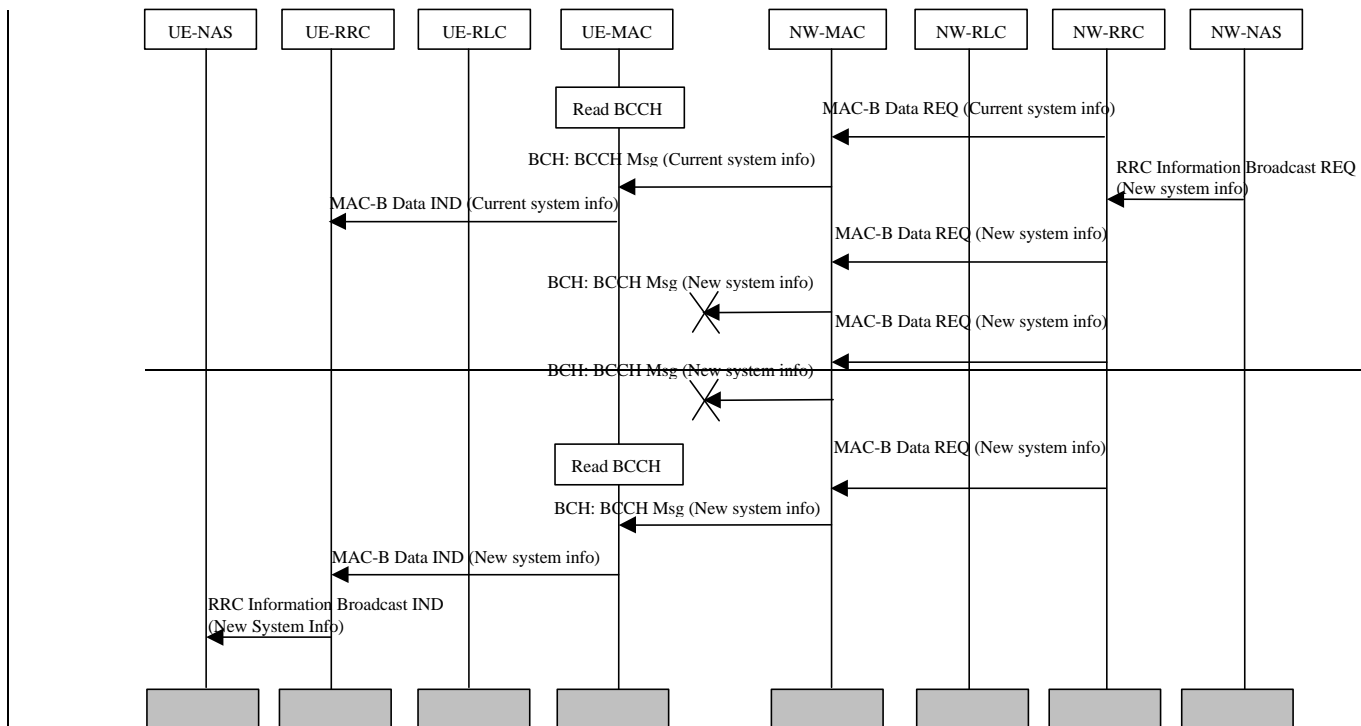
Figure 5. Example sequence, non-access stratum initiated change of broadcast system info.
