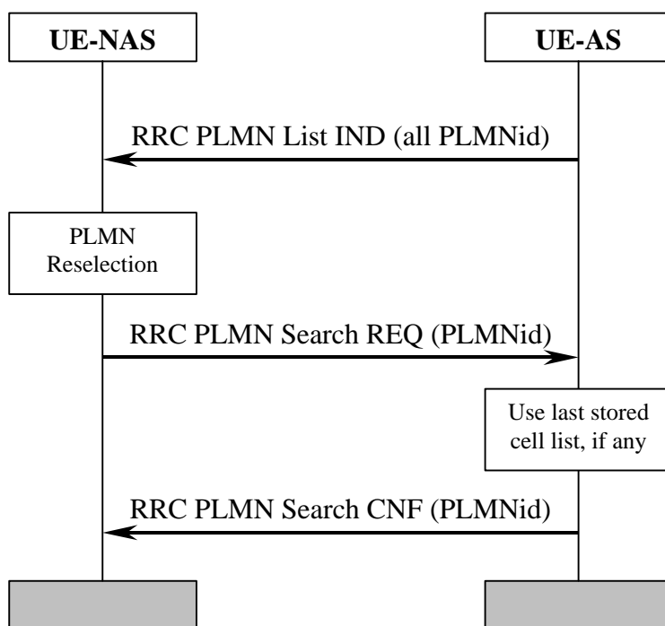
Figure 9. PLMN Reselection, automatic mode.
