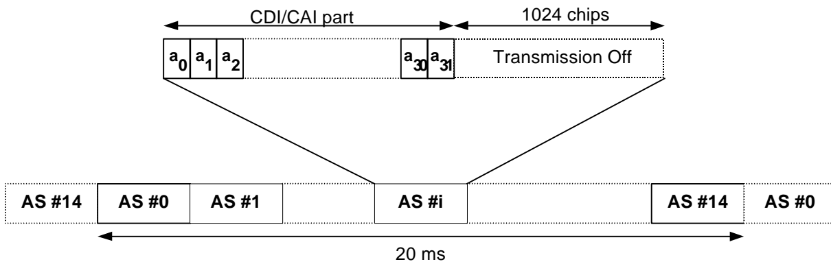
Figure 21: Structure of CD/CA Indicator Channel (CD/CA-ICH)
