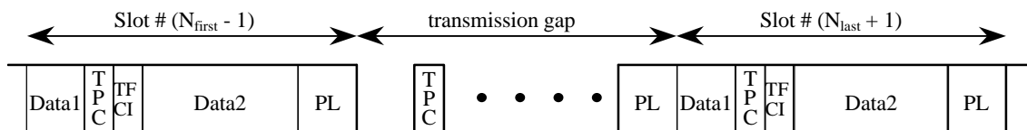
(b) Frame structure type B
