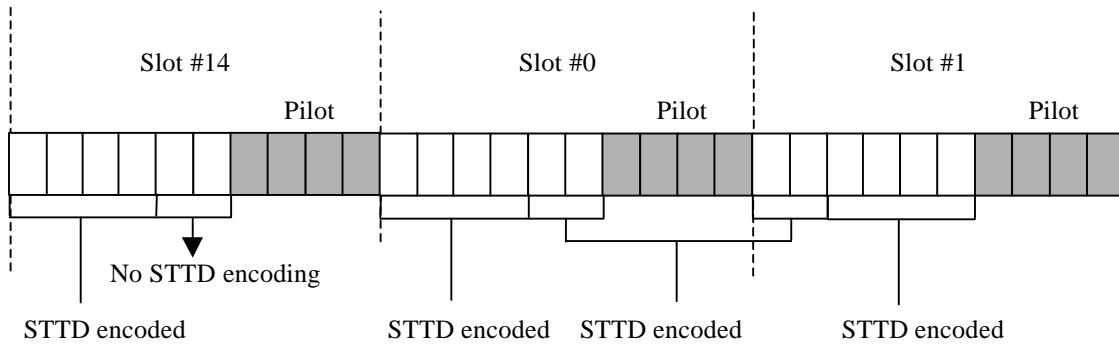
Figure 10: STTD encoding for SF = 512 DPCH
