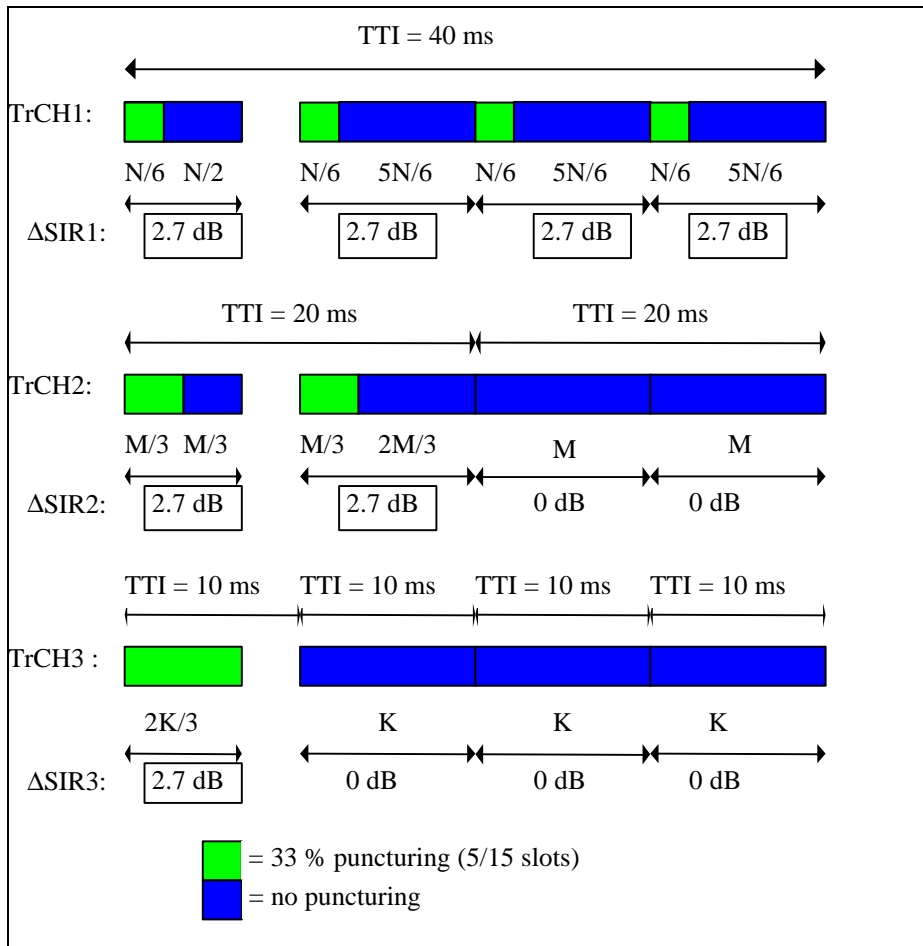
Figure 1. Puncturing done per radio frame basis. Shows how the bits are spread to different frames after 1 st interleaving.
