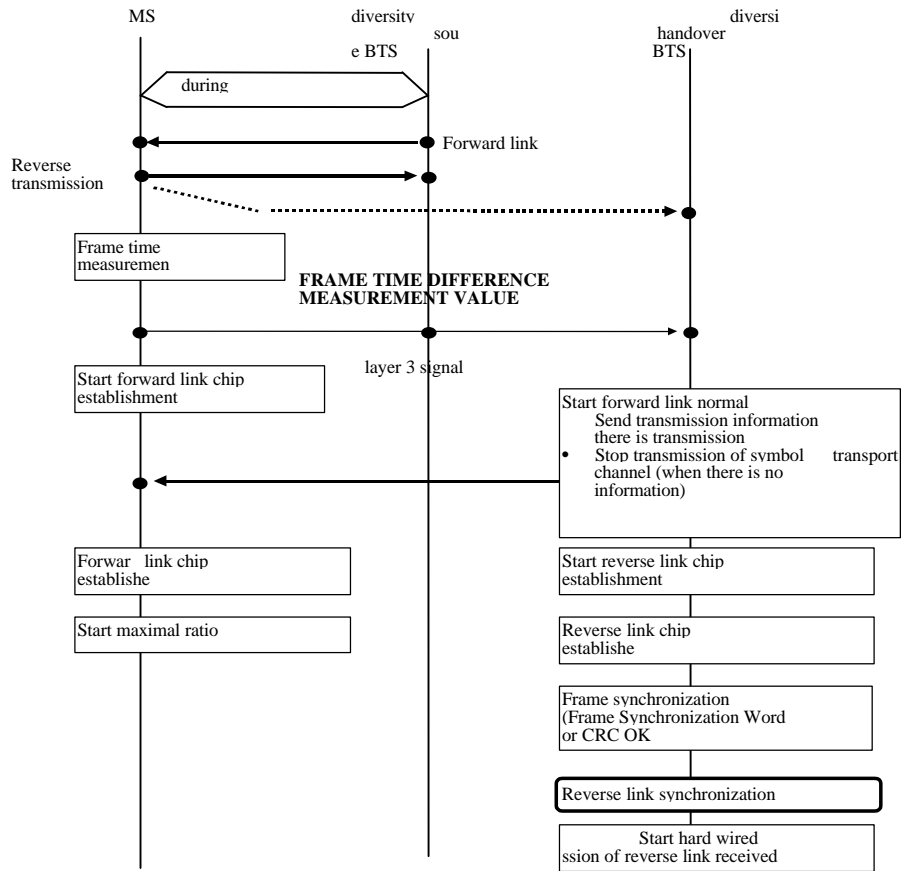
Fig. 4 Figure 3 Synchronisation Establishment Flow Upon Intra/Inter-cell Diversity Handover
