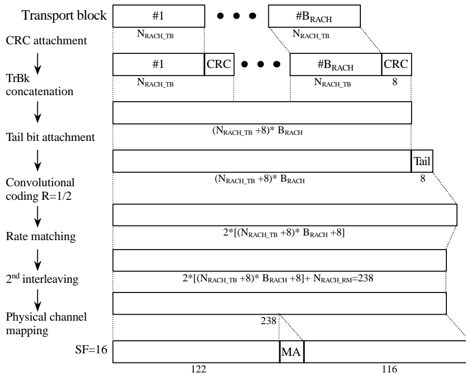
Figure 31: Channel coding and multiplexing example for RACH
