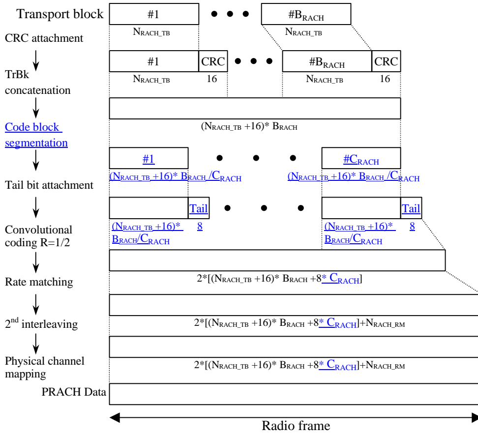
Figure 11: Channel coding and multiplexing example for PRACH
