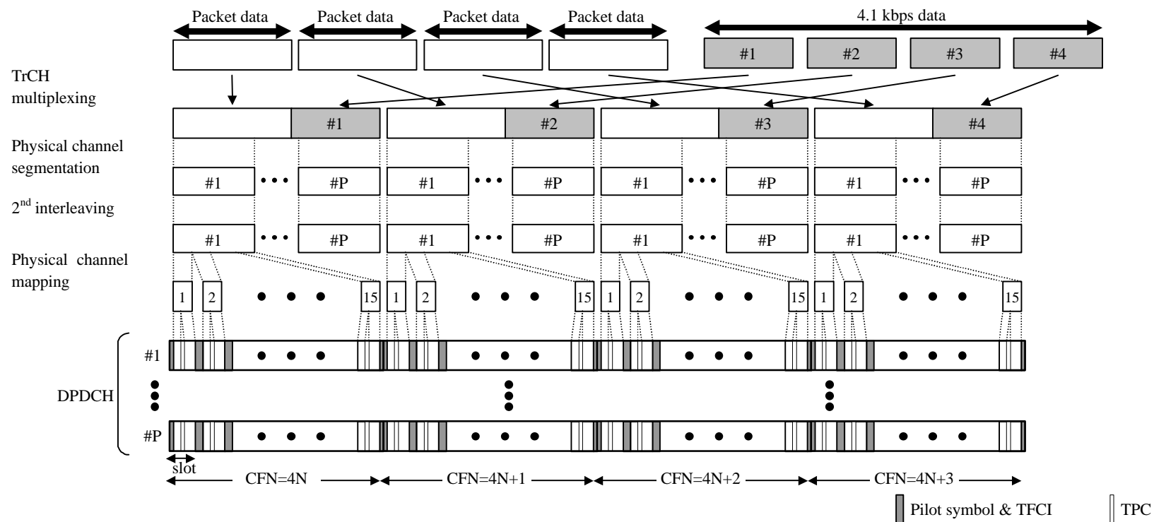
Figure 9: Channel coding and multiplexing example for multiplexing of 64/128/384 kbps packet data and 4.1 kbps data
