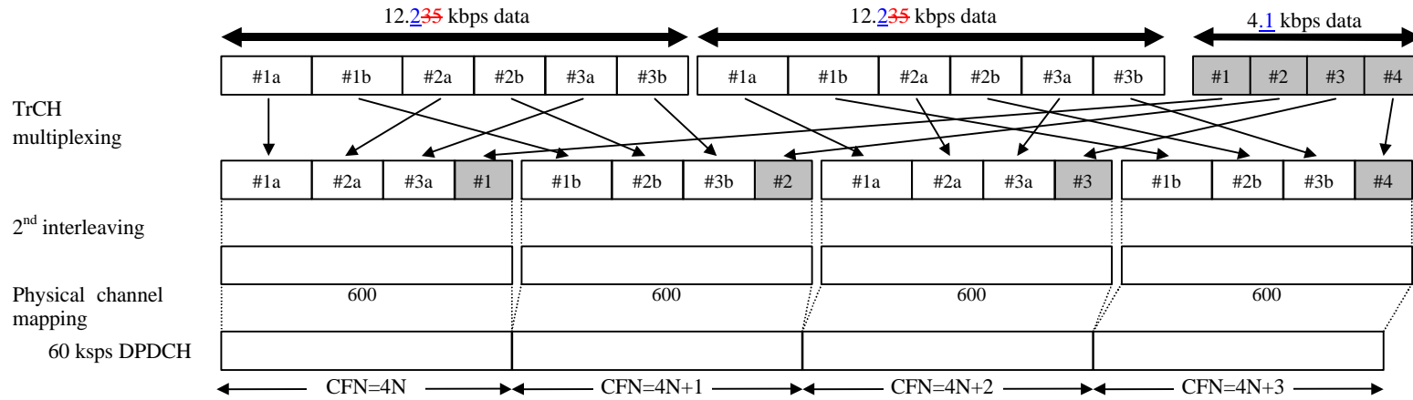
Figure 17: Channel coding and multiplexing example for multiplexing of 12.235 kbps data and 4.1 kbps data
