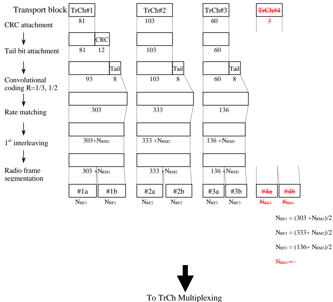
Figure 4: Channel coding and multiplexing example for 12.235 kbps data
