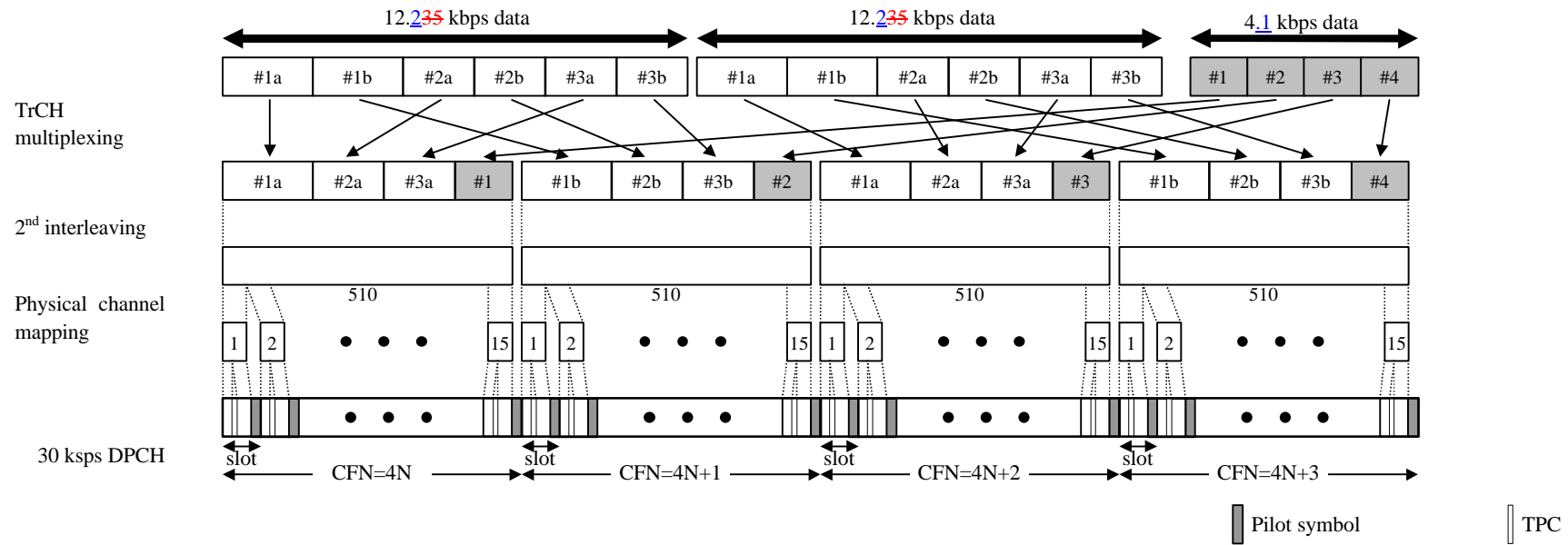
Figure 8: Channel coding and multiplexing example for multiplexing of 12.235 kbps data and 4.1 kbps data
