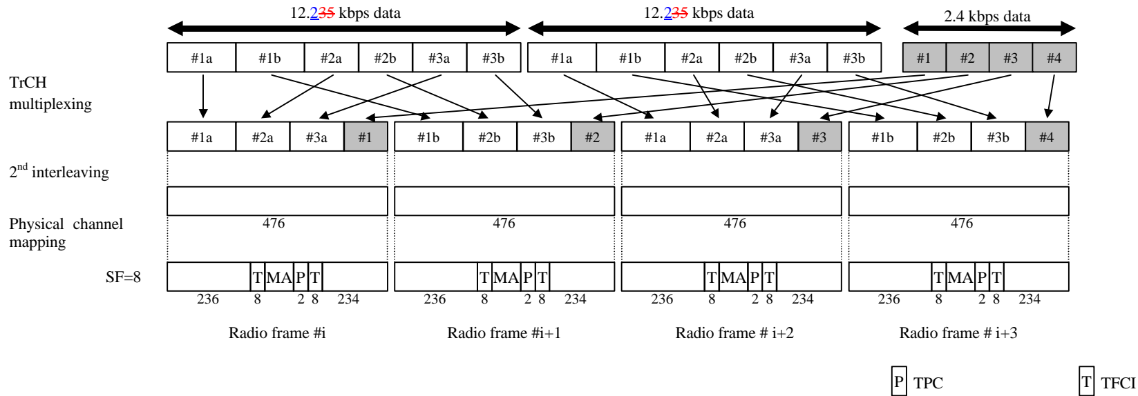
Figure 33: Channel coding and multiplexing example for multiplexing of 12.235 kbps data and 2.4 kbps data
