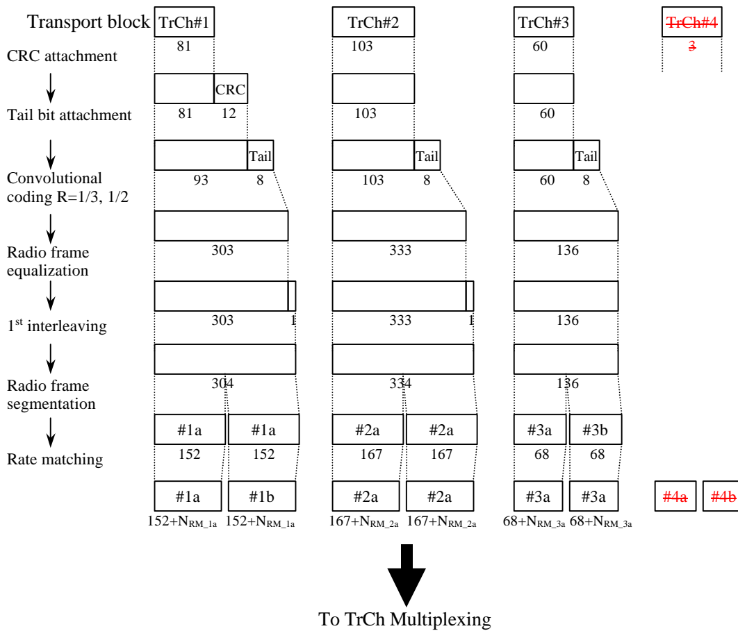
Figure 24: Channel coding and multiplexing example for 12.235 kbps data
