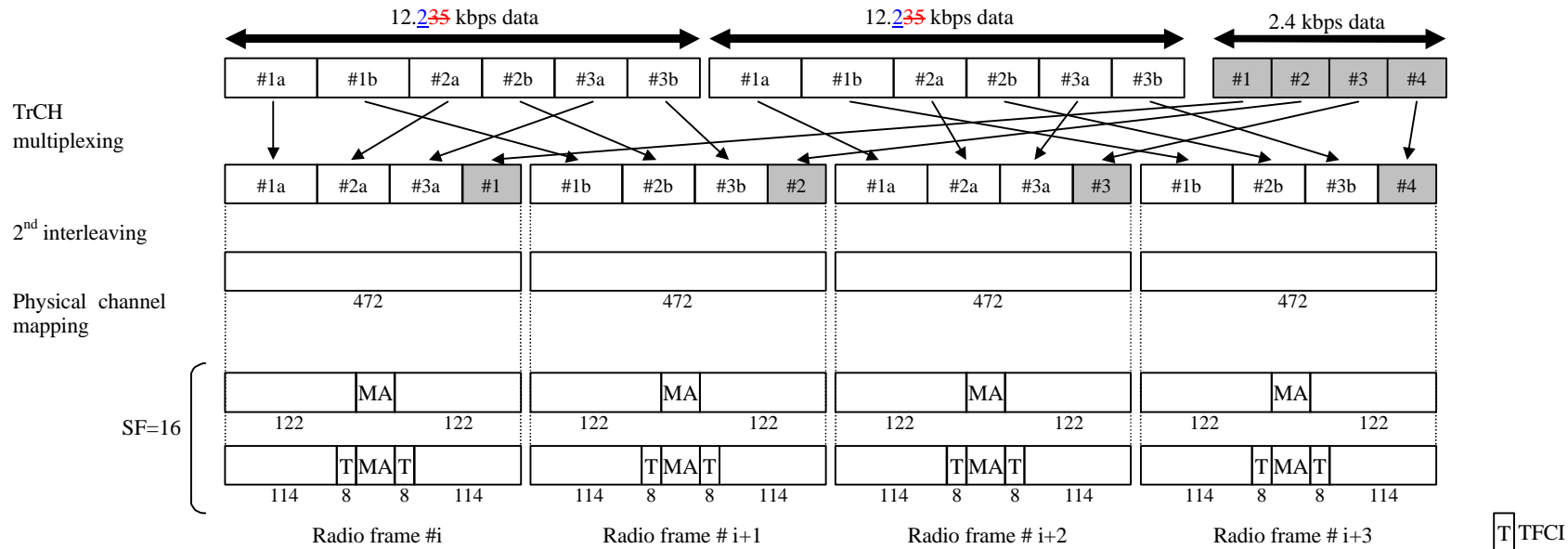
Figure 28: Channel coding and multiplexing example for multiplexing of 12.235 kbps data and 2.4 kbps data
