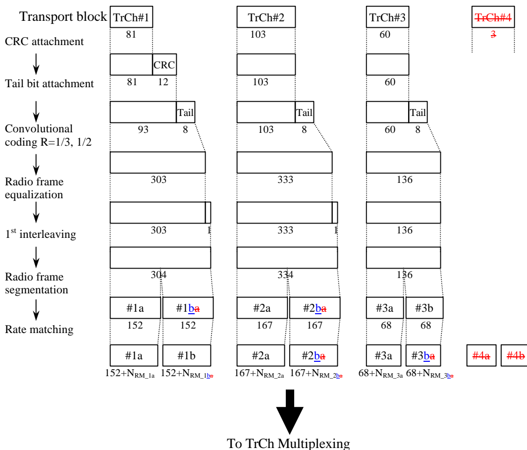
Figure 13: Channel coding and multiplexing example for 12.235 kbps data
