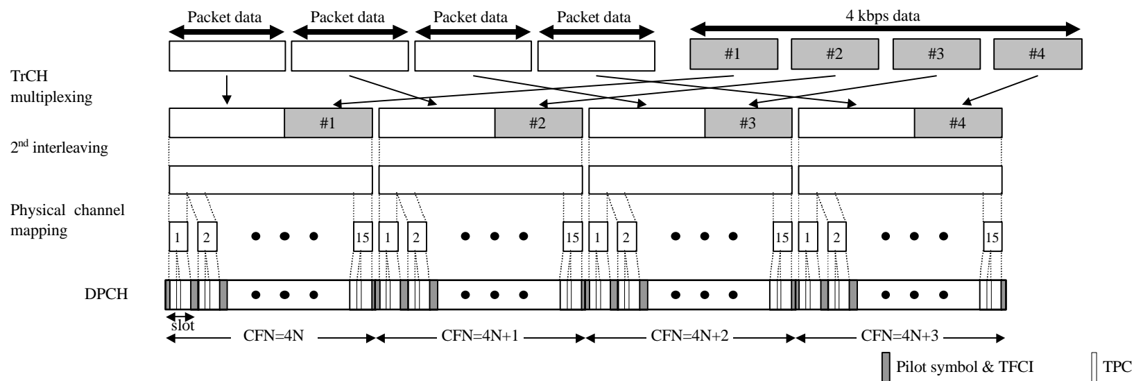
Figure 9: Channel coding and multiplexing example for multiplexing of 64/128/384 kbps packet data and 4 kbps data
