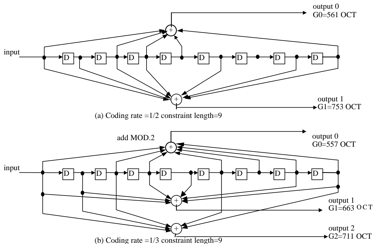
Figure 3: Convolutional Coder
