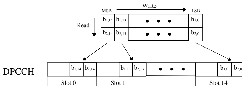
Figure 13: Mapping of TFCI code words to the slots of the radio frame in Split Mode
