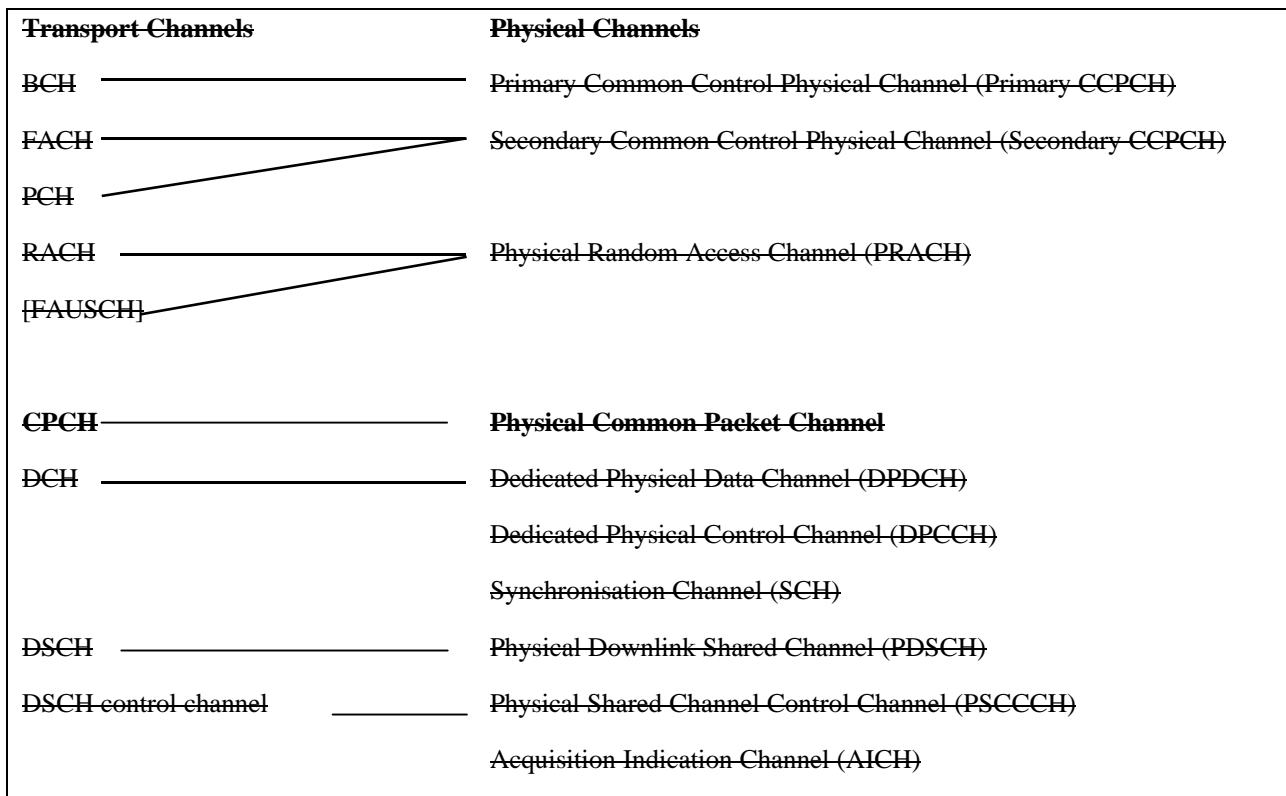
Figure 4: Transport-channel to physical-channel mapping.
