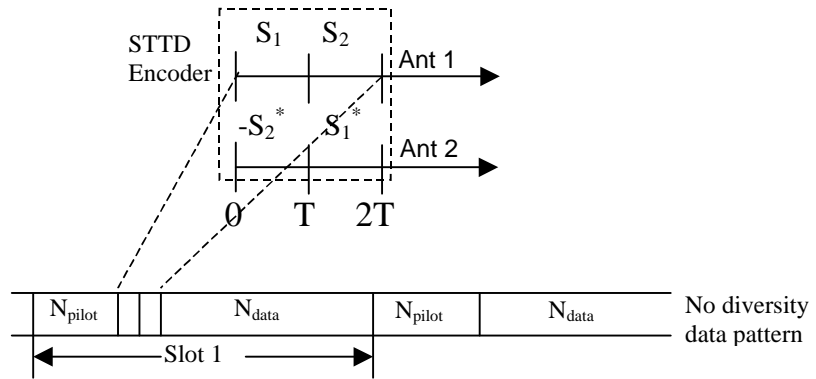
Figure 88: Block diagram of STTD encoder. The symbols S_1 , S_2 are QPSK symbols and T denotes the symbol time.
