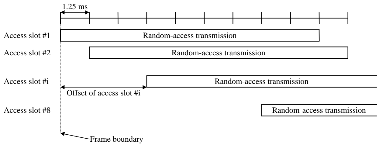
Figure 22: PRACH allocated for RACH access slots.
