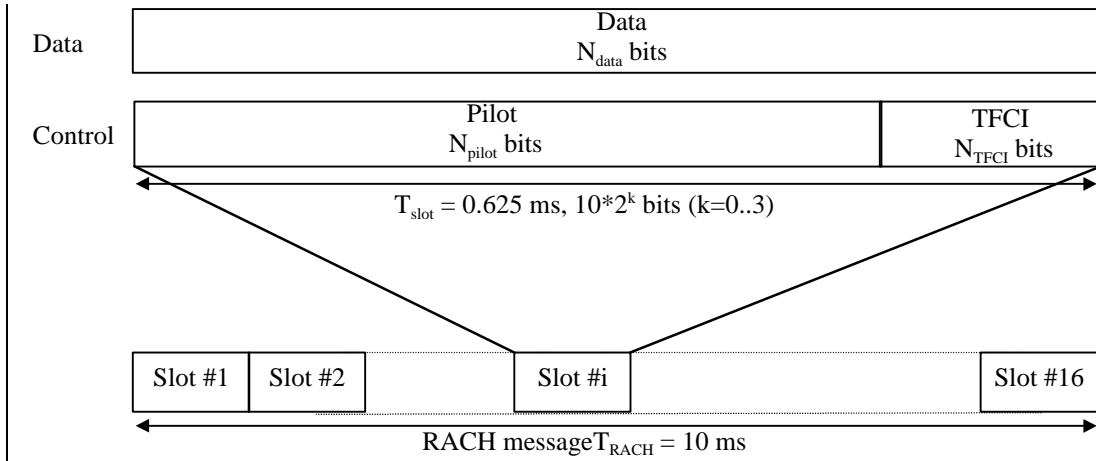
Figure 55: The message part of the random-access burst.
