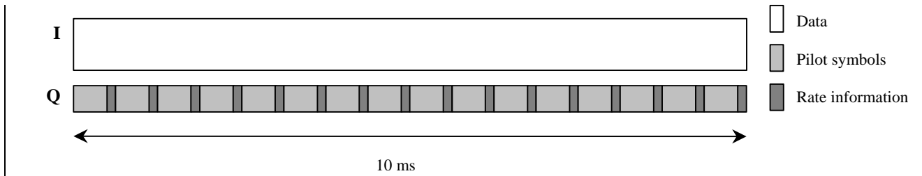
Figure 44: The message part of the random-access burst.
