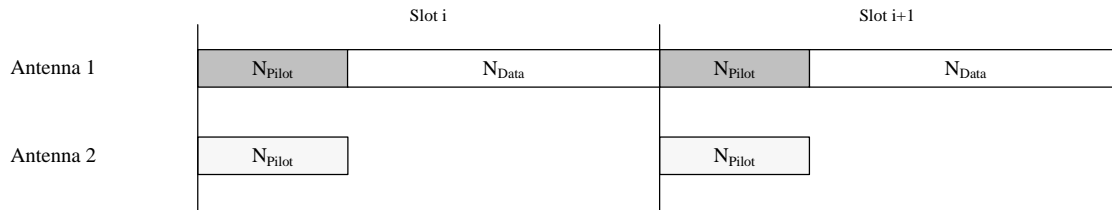
Figure 1343: Slot structure of Primary CCPCH when diversity transmission is applied on dedicated channels.
