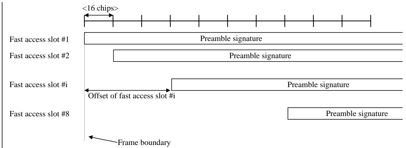
Figure 66: PRACH used for FAUSCH fast access slots.
