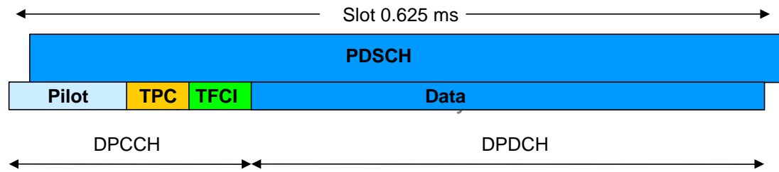
Figure 1747: Frame structure for the DSCH when associated to a DCH.
