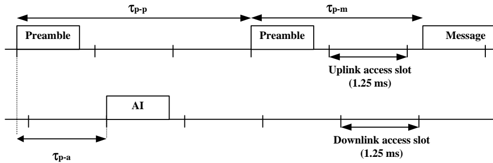
Figure 2323: Timing of PRACH and AICH transmission
