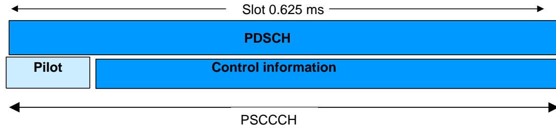
Figure 1848: Frame structure for the DSCH when associated to a DSCH control channel.
