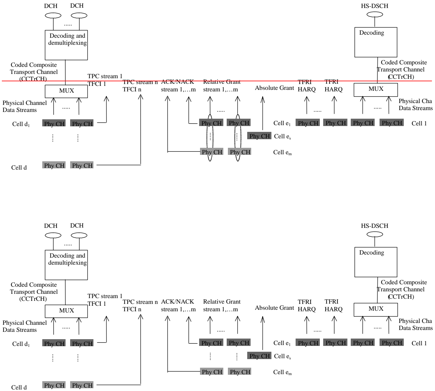
Figure 6.3.2-1: Model of the UE's Downlink physical layer. HS-DSCH serving cell is cell 1 in this figure
