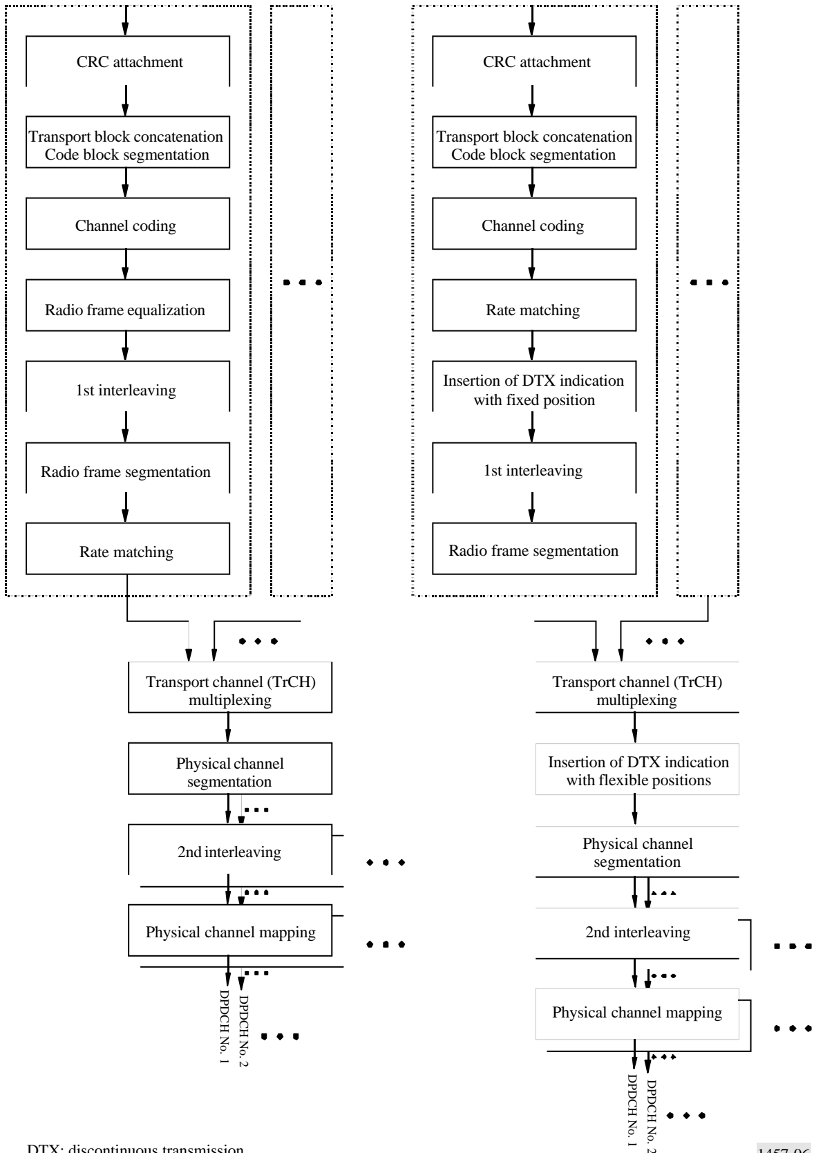
FIGURE 6 DCH transport channel multiplexing structure (left: uplink; right: downlink)
