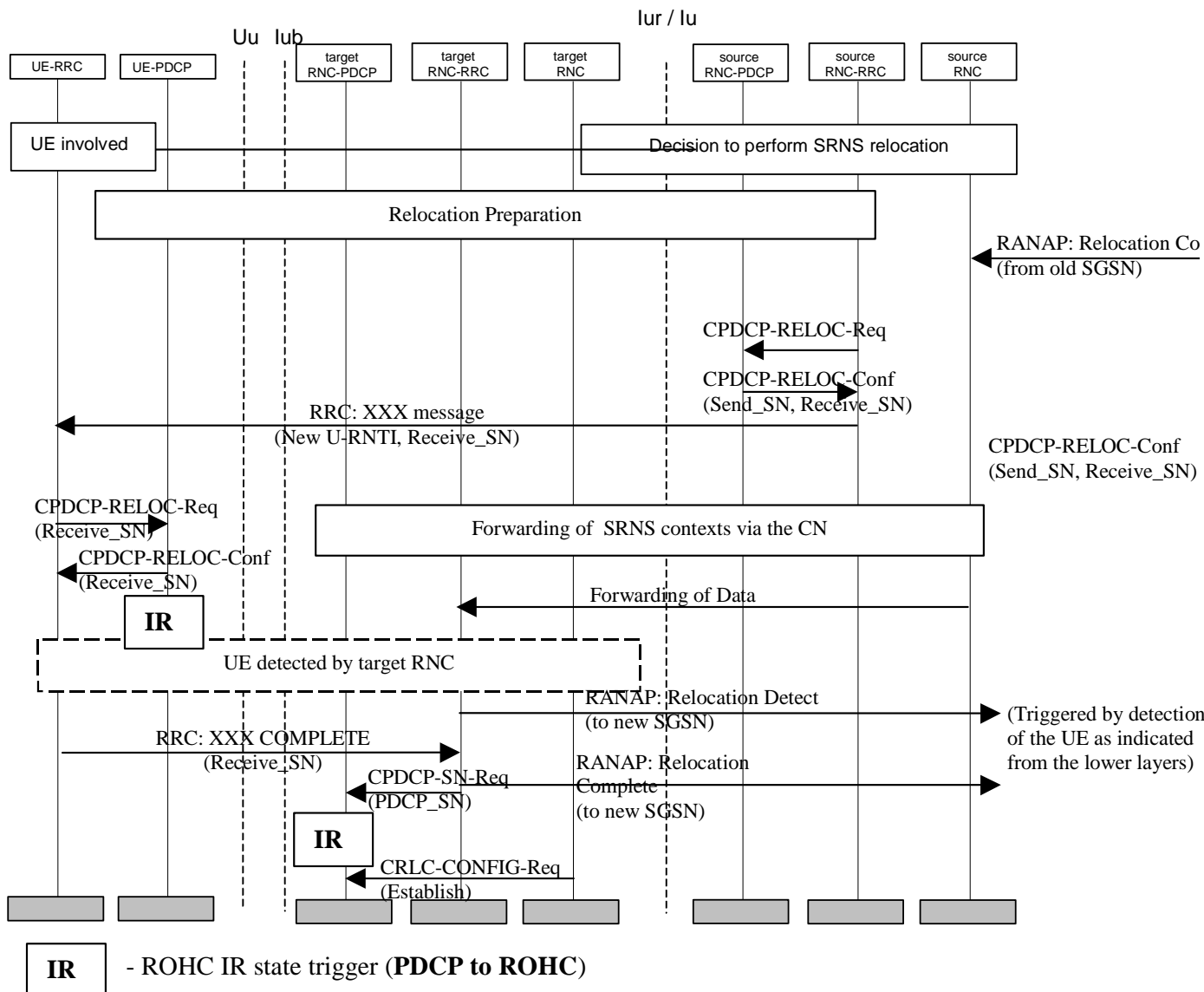
Figure 12: ROHC handling during Hard Handover with SRNS relocation
