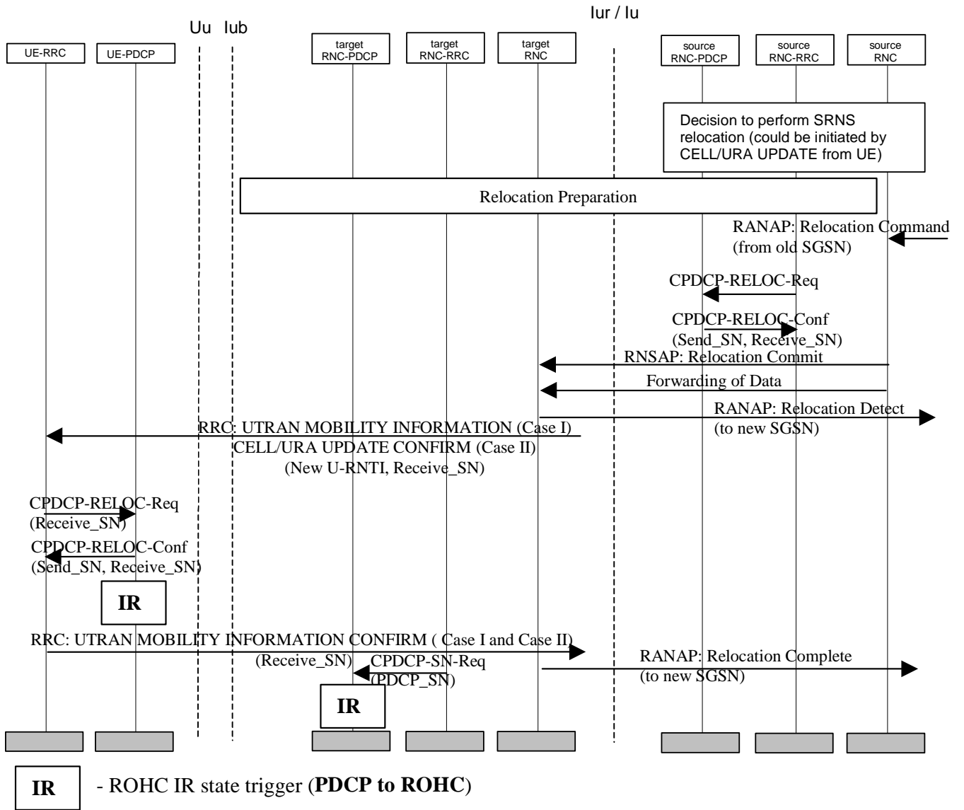
Figure 11: ROHC handling during SRNS relocation
