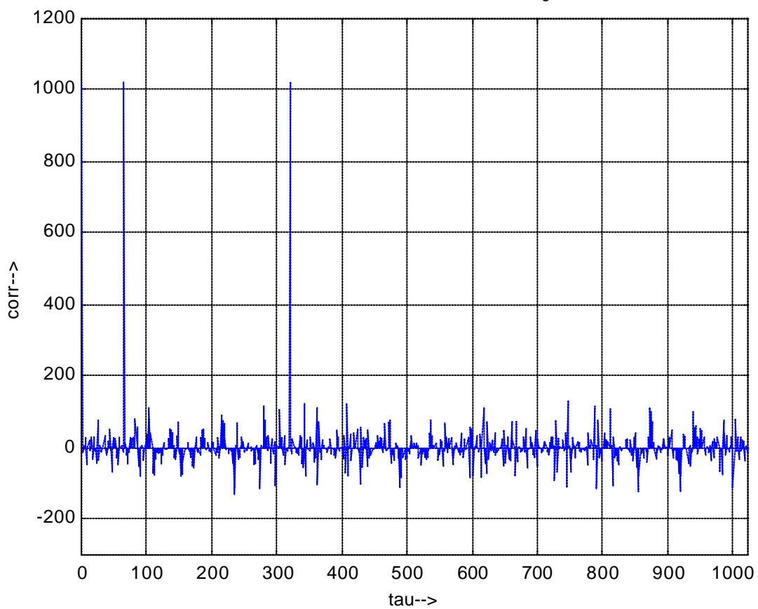
Output of cyclic correlator for \phi_g(n)
