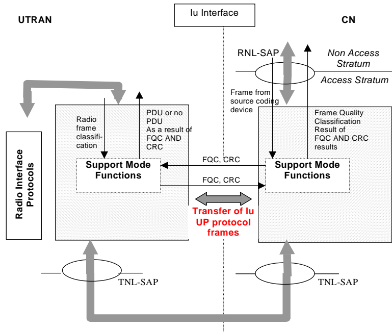
Figure 65: Frame quality classification in Iu UP
