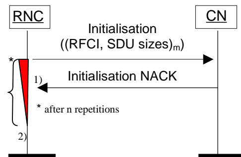
Figure 109: Unsuccessful initialisation of Iu UP: 1) n negative acknowledgement or 2) n timer expires
