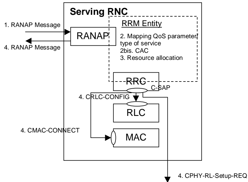
Figure 6-1: This model shows how standardized RANAP and RRC layers are involved in the CAC process.
