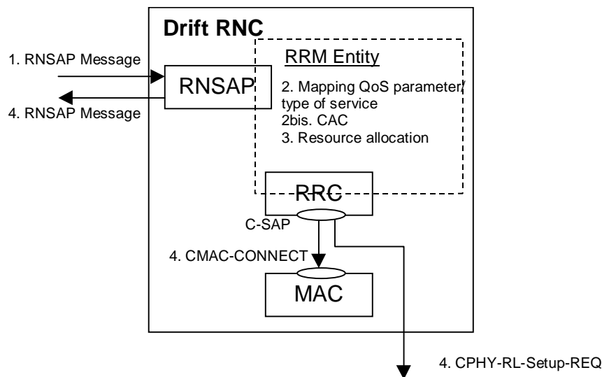
Figure 6-3: This model shows how standardized RNSAP and RRC layers are involved in the CAC process.
