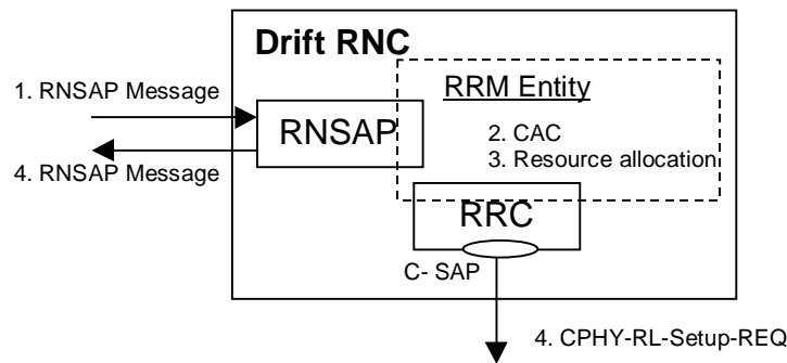
Figure 6-2: This model shows how standardized RNSAP and RRC layers are involved in the CAC process.
