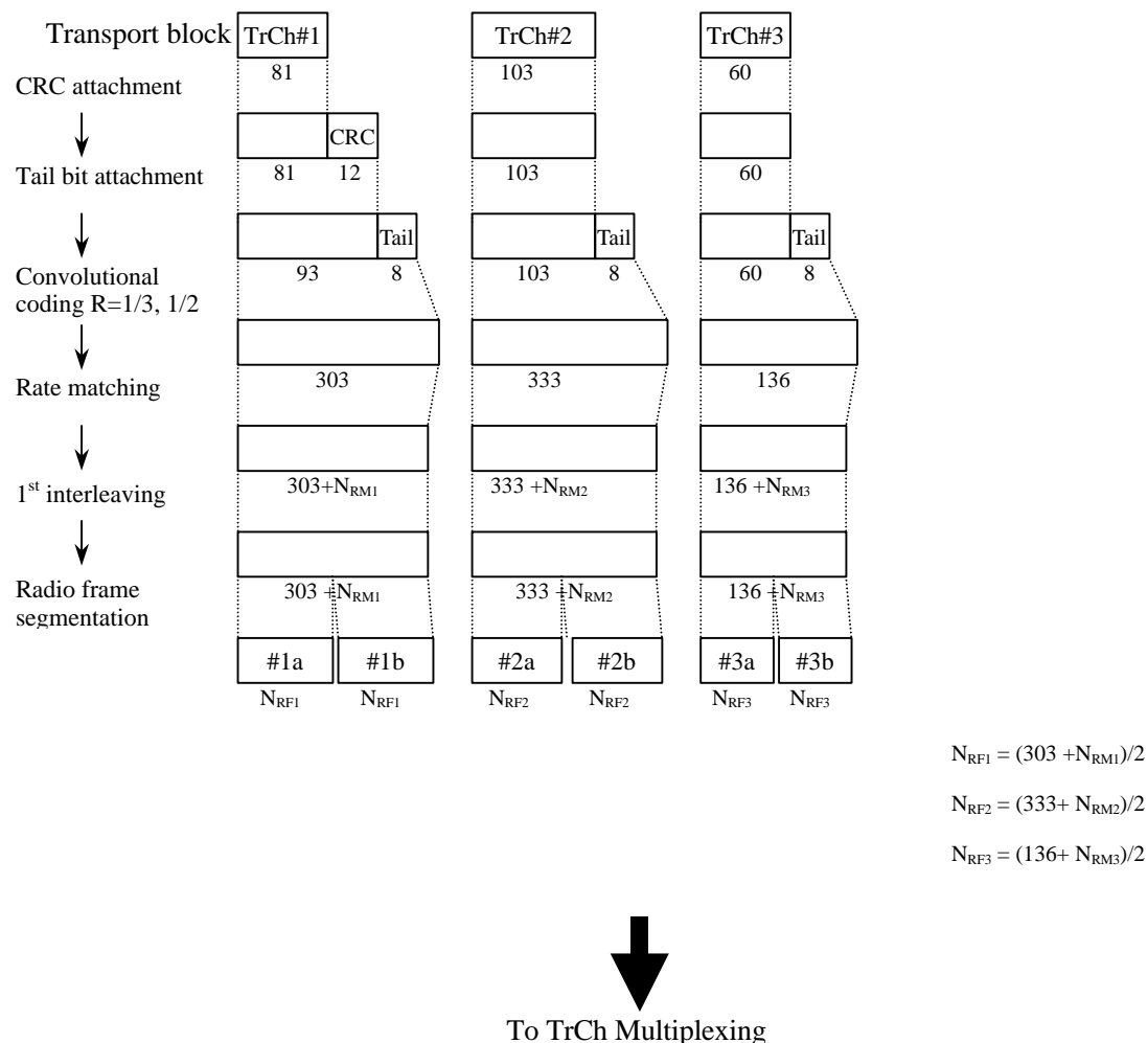
Figure 4: Channel coding and multiplexing example for 12.2 kbps data
