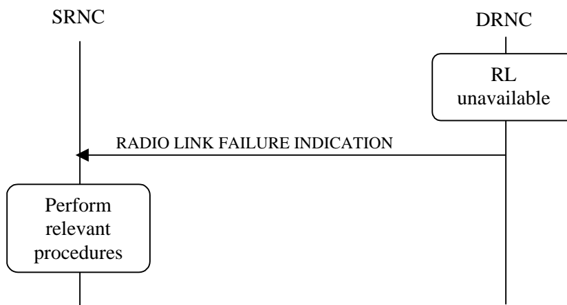
Figure 9-11. RL Failure procedure
