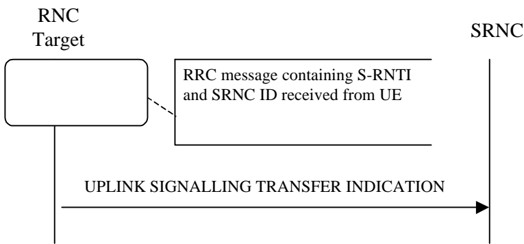
Figure 9-8: An example RNSAP message flow at I ur interface for Uplink Signalling Transfer
