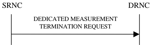
Figure 9-x: Measurement Termination Procedure initiated by SRNC
