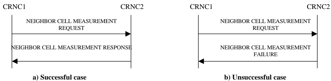
Figure 9-x: An example RNSAP message flow at I_{ur} interface for Neighbour Cell Measurement.
