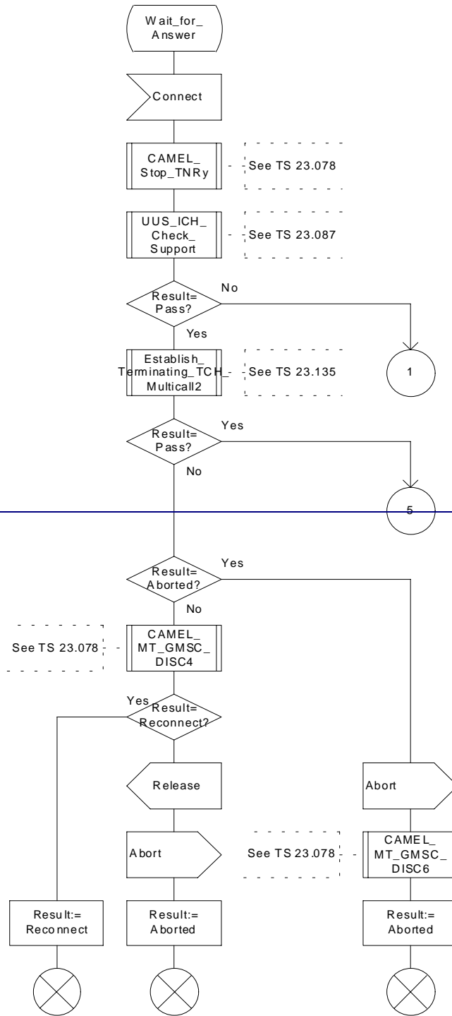
Figure 69f: Procedure Complete_Call_In_MSC (sheet 6)
