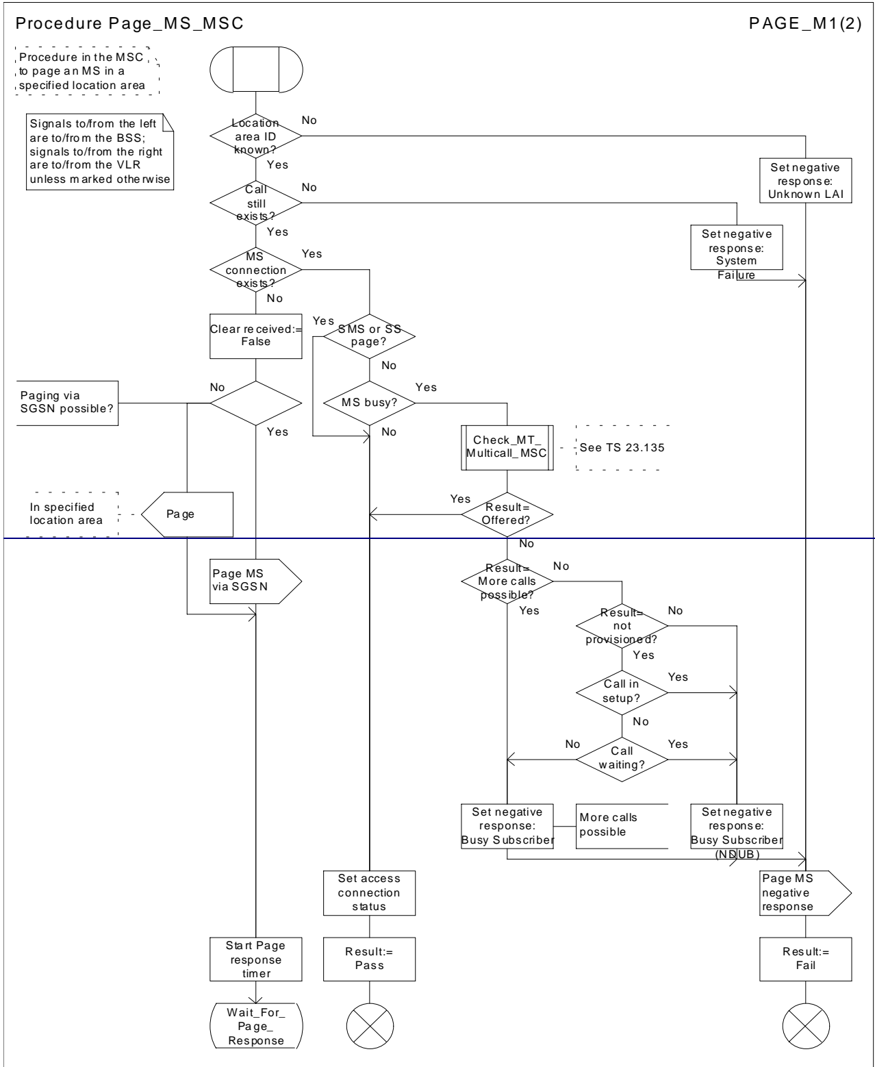
Figure 2a: Procedure Page_MS_MSC (sheet 1)
