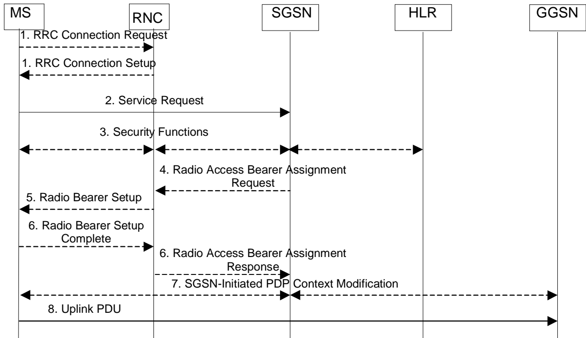
Figure 1446: Service Request Initiated by MS Procedure
