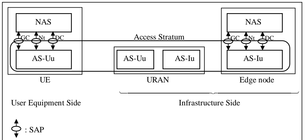
Figure 2: Service Access Points (SAPs) offered by the Access Stratum (AS)
