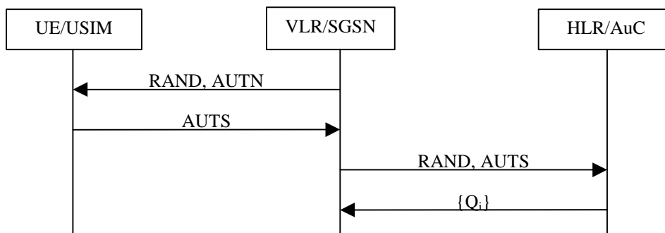
Figure 12: Resynchronization mechanism
