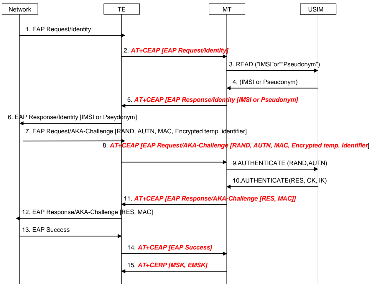
Figure 12 1 : Full authentication with EAP AKA
