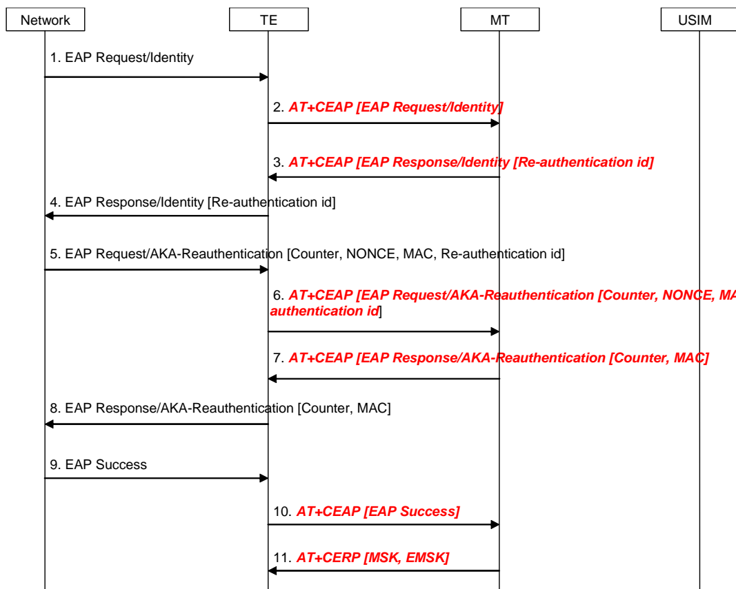
Figure 163: Fast re-authentication with EAP AKA
