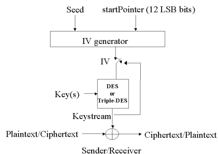
Figure A.7: The encryption/decryption function
