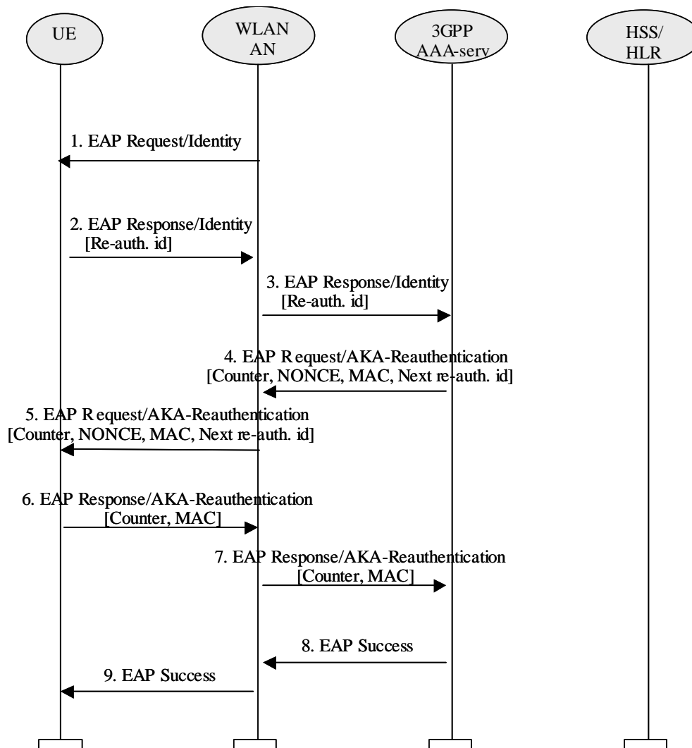
Figure 7.3 : EAP AKA Re-authentication
