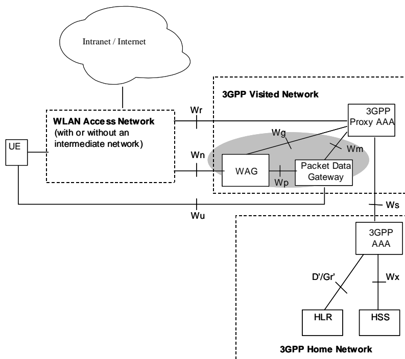
Figure 4.3 Roaming reference model, services in the VPLMN
