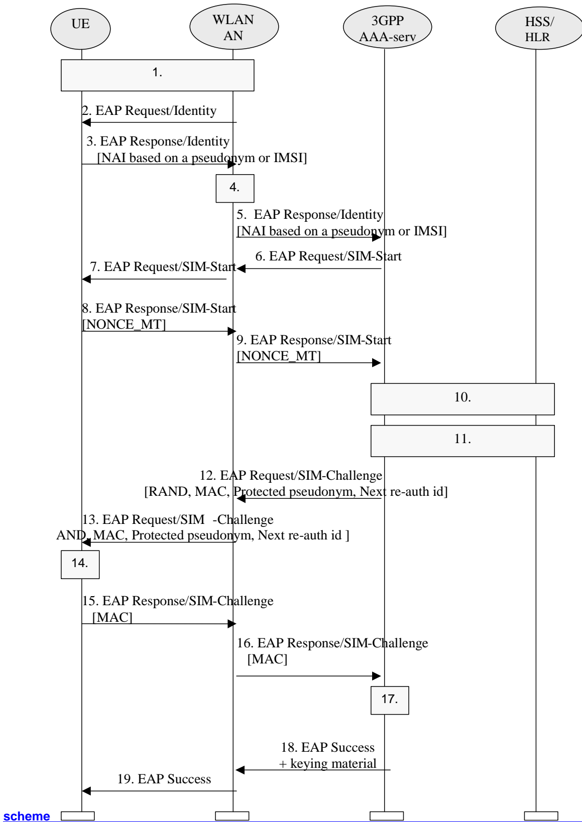
7.2: Authentication based on EAP SIM scheme
