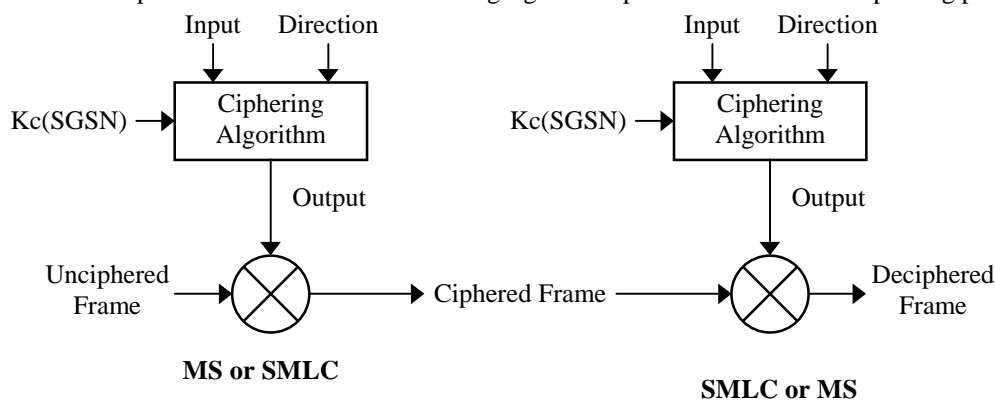
Figure 3 LCS ciphering environment
