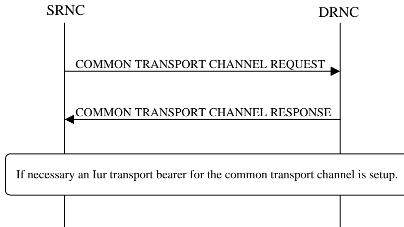
Figure 209-x: An example RNSAP message flow at I ur interface for Common Transport Channel Initialization.
