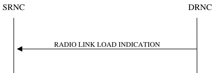
Figure 139-x: An example RNSAP message flow at I ur interface for Radio Link Load Indication.
