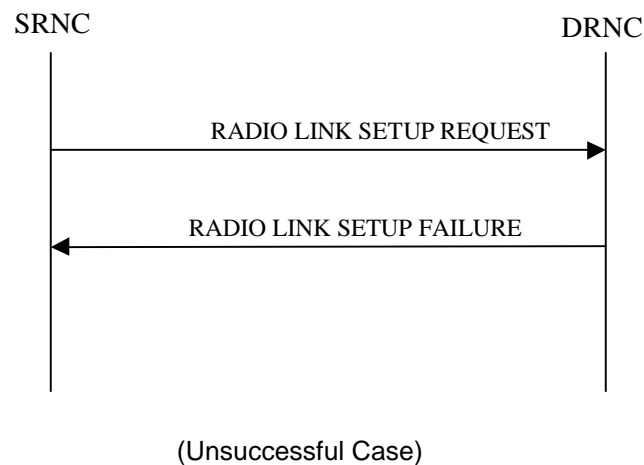
Figure 59-4: An example RNSAP message flow at I ur interface for RL setup.
