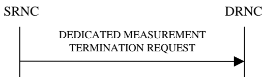
Figure 169-x: Measurement Termination Procedure initiated by SRNC
