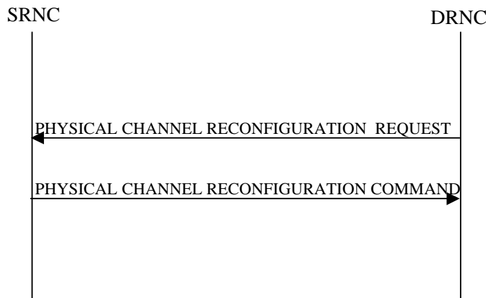
Figure 109-6-: Physical Channel Reconfiguration procedure
