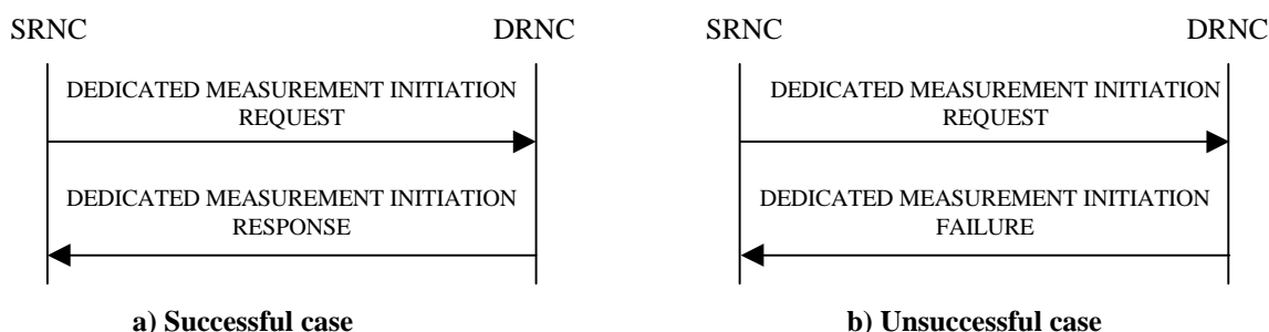
Figure 149-x: Measurement Request Procedure
